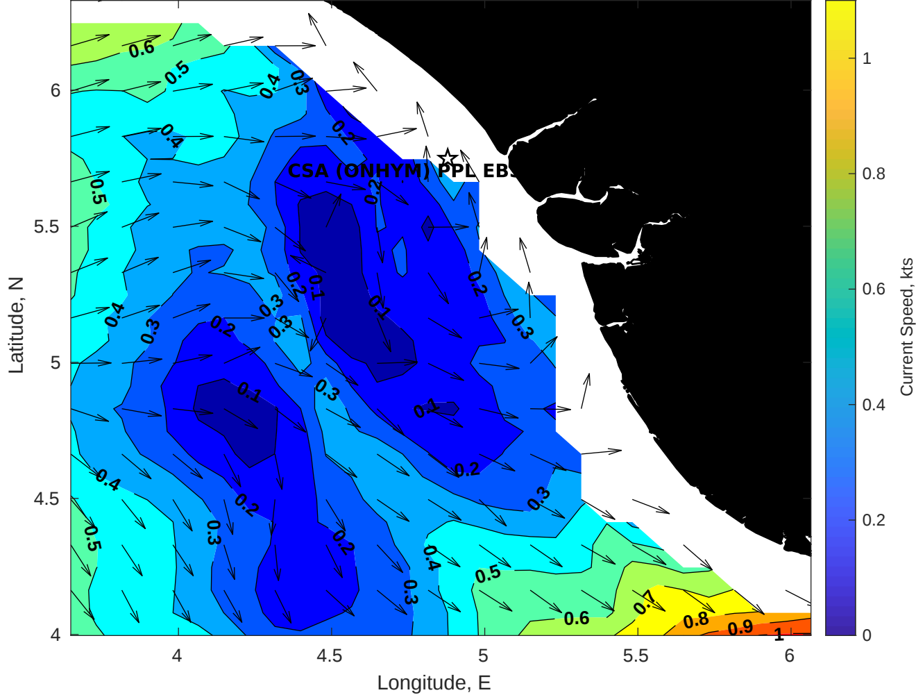
Surface Currents for CSA (ONHYM) PPL EBS - Nigeria at 23-Dec-2025 00:00:00
