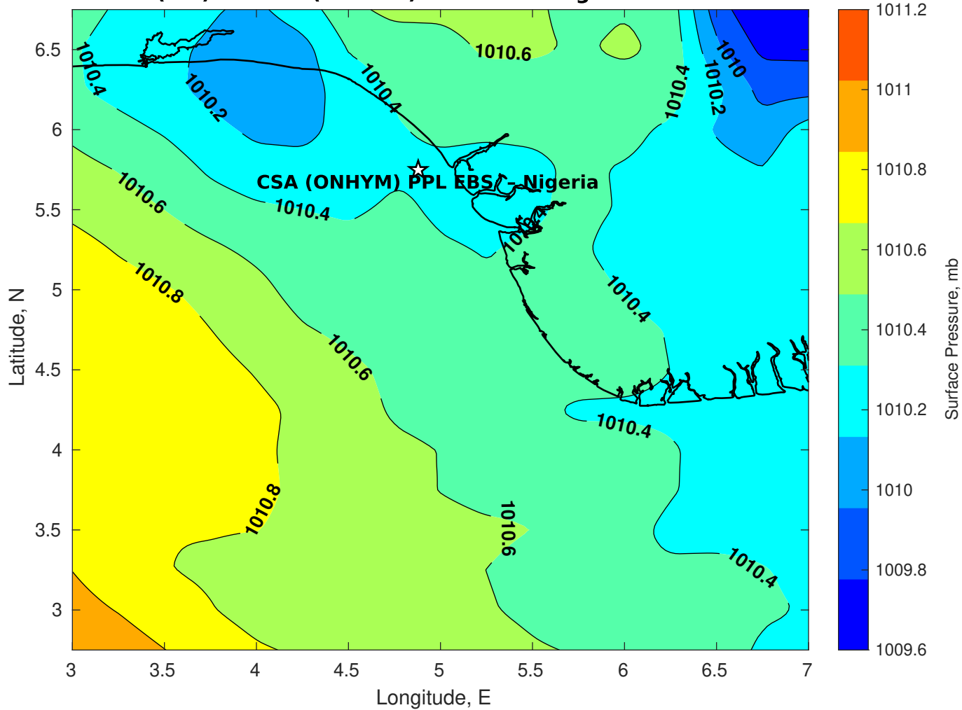
Surface Pressure (mb) for CSA (ONHYM) PPL EBS - Nigeria at 24-Dec-2025 00:00:00
