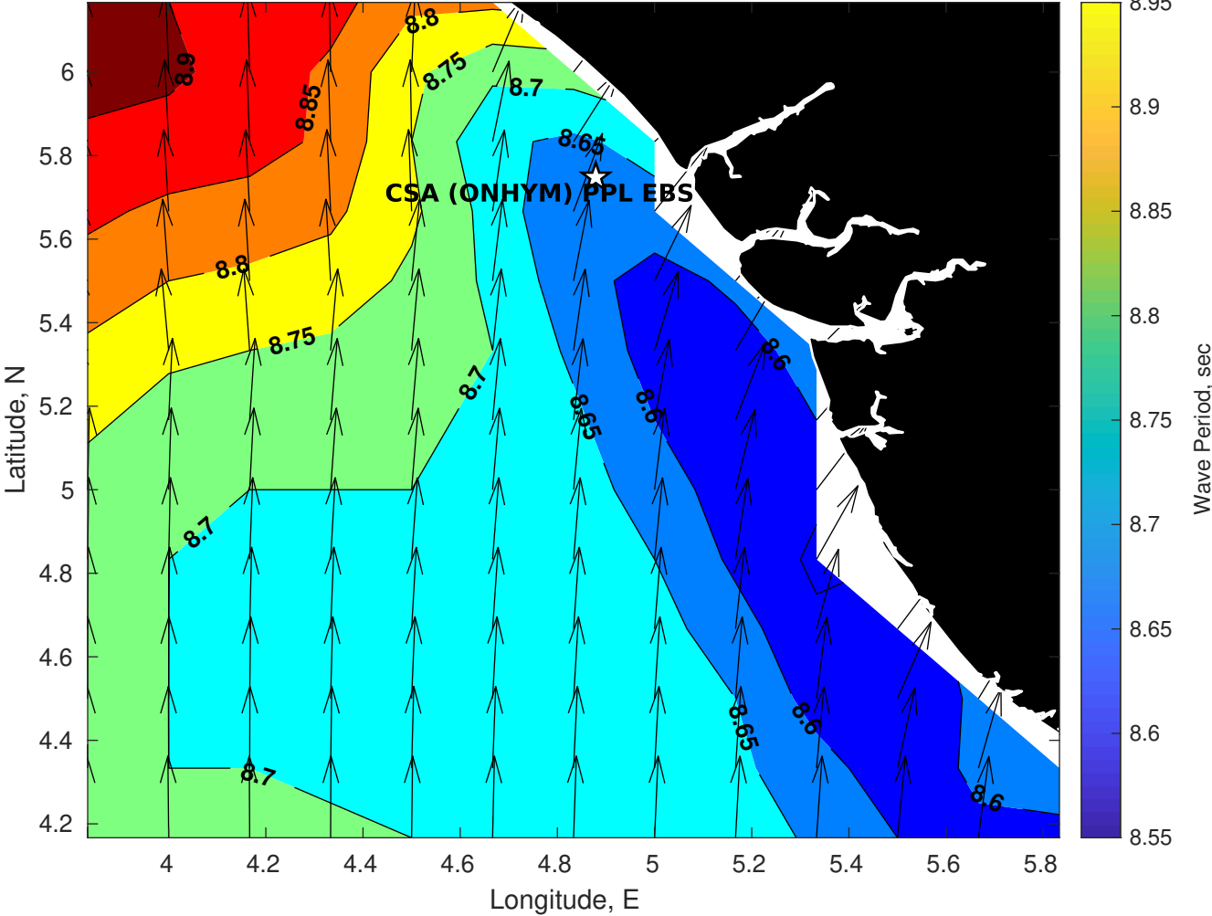
GFS Wave Period (sec) for CSA (ONHYM) PPL EBS - Nigeria at 24-Dec-2025 09:00:00
