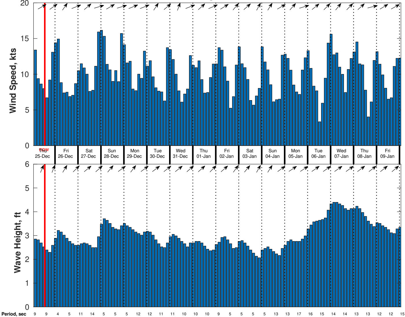
Wind & Wave Forecast for CSA (ONHYM) PPL EBS - Nigeria from 24-Dec-2025 02:00:00 to 09-Jan-2026 02:00:00
