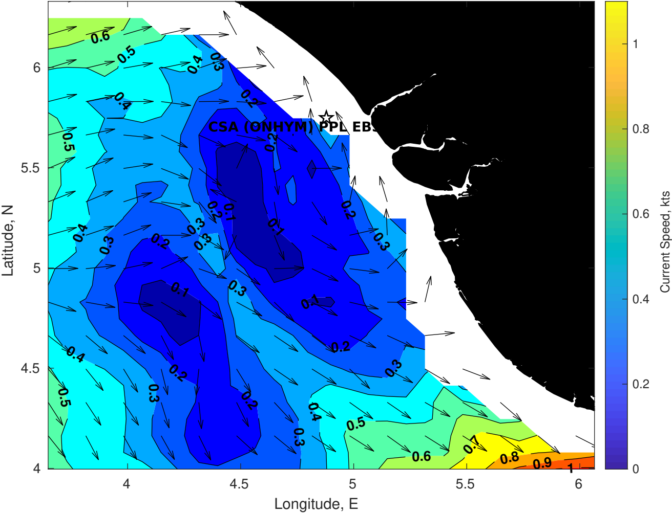
Surface Currents for CSA (ONHYM) PPL EBS - Nigeria at 23-Dec-2025 00:00:00
