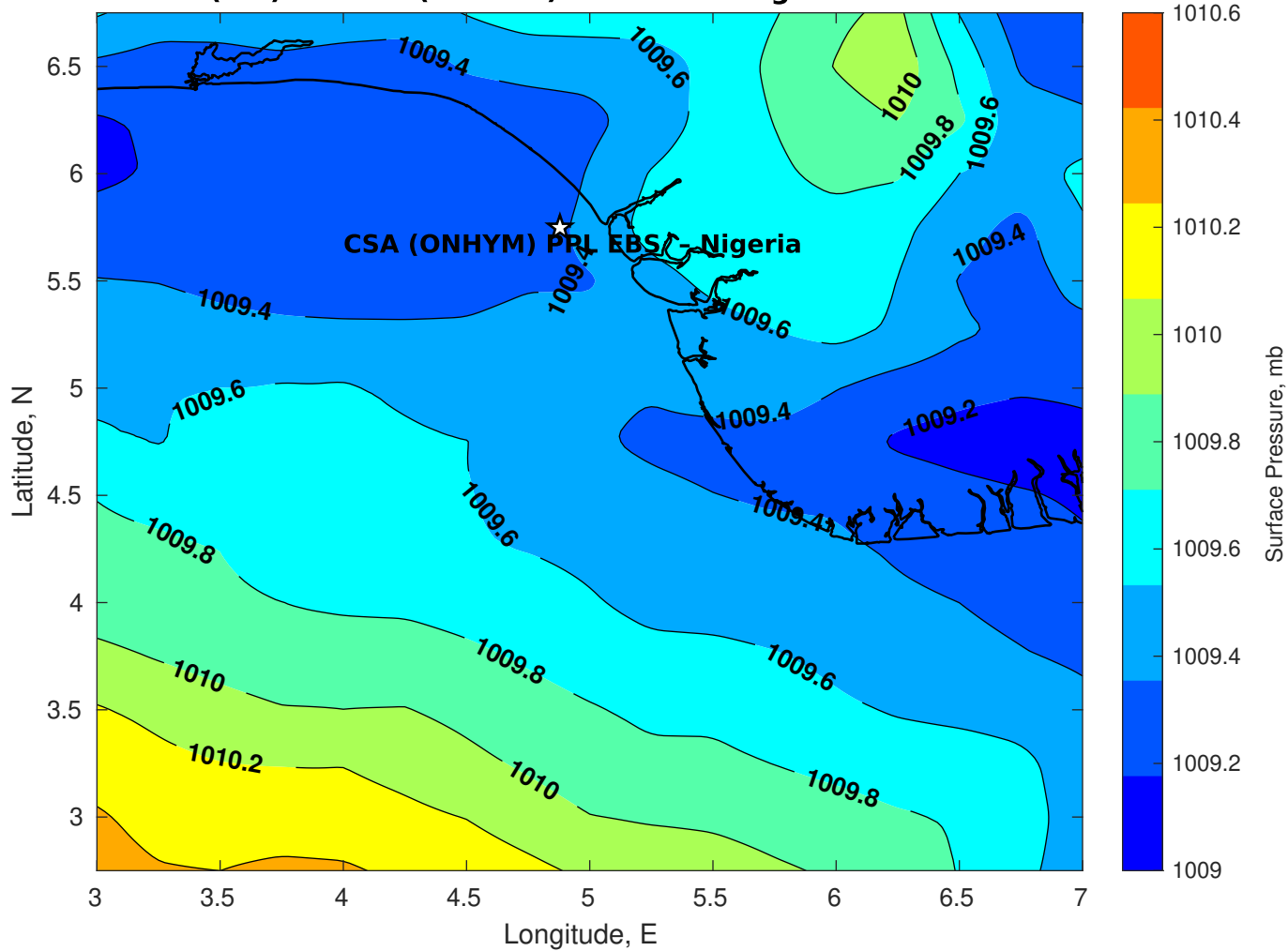
Surface Pressure (mb) for CSA (ONHYM) PPL EBS - Nigeria at 26-Dec-2025 00:00:00
