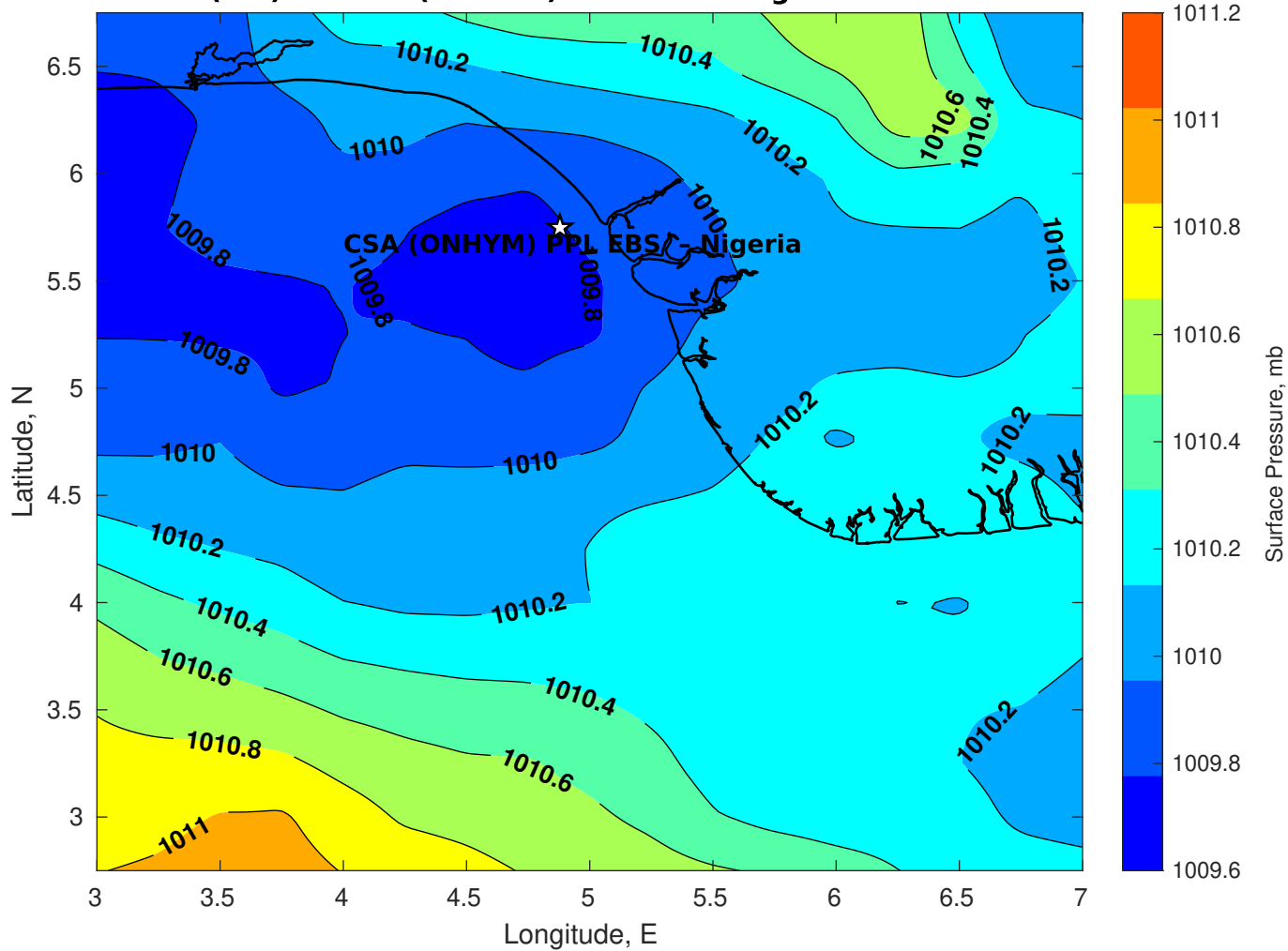
Surface Pressure (mb) for CSA (ONHYM) PPL EBS - Nigeria at 25-Dec-2025 00:00:00
