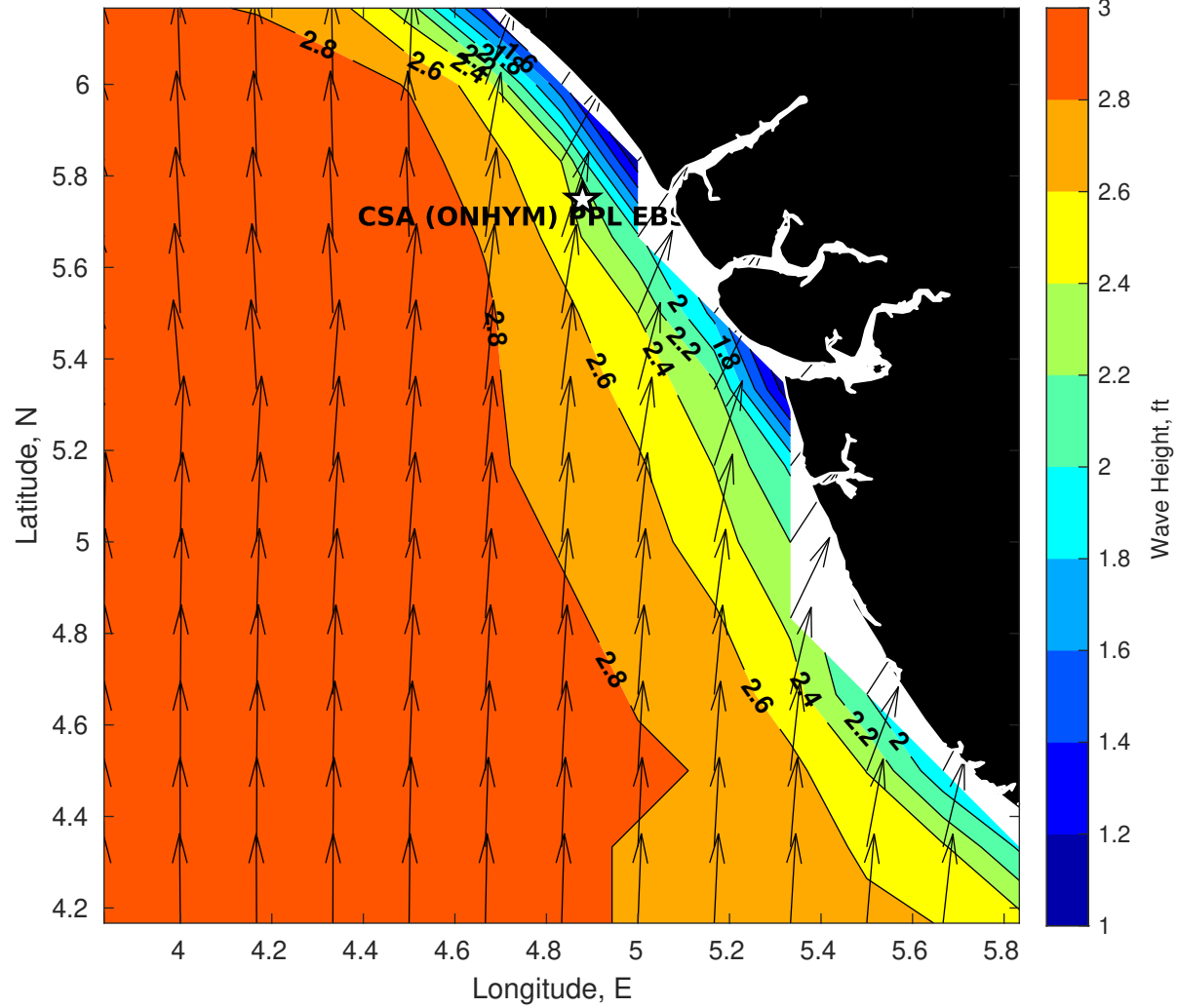
GFS Wave Height (ft) for CSA (ONHYM) PPL EBS - Nigeria at 24-Dec-2025 09:00:00
