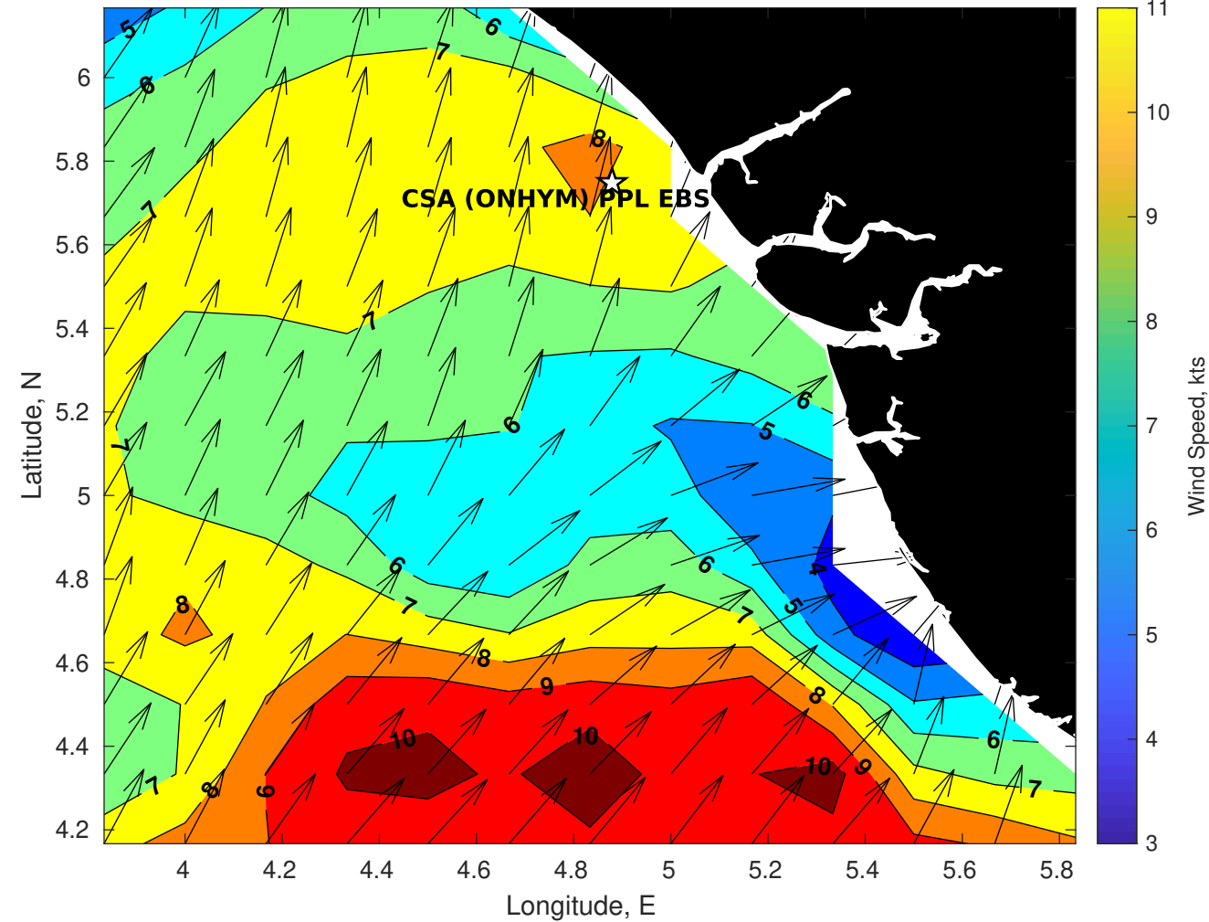
GFS Winds (kts) for CSA (ONHYM) PPL EBS - Nigeria at 24-Dec-2025 09:00:00
