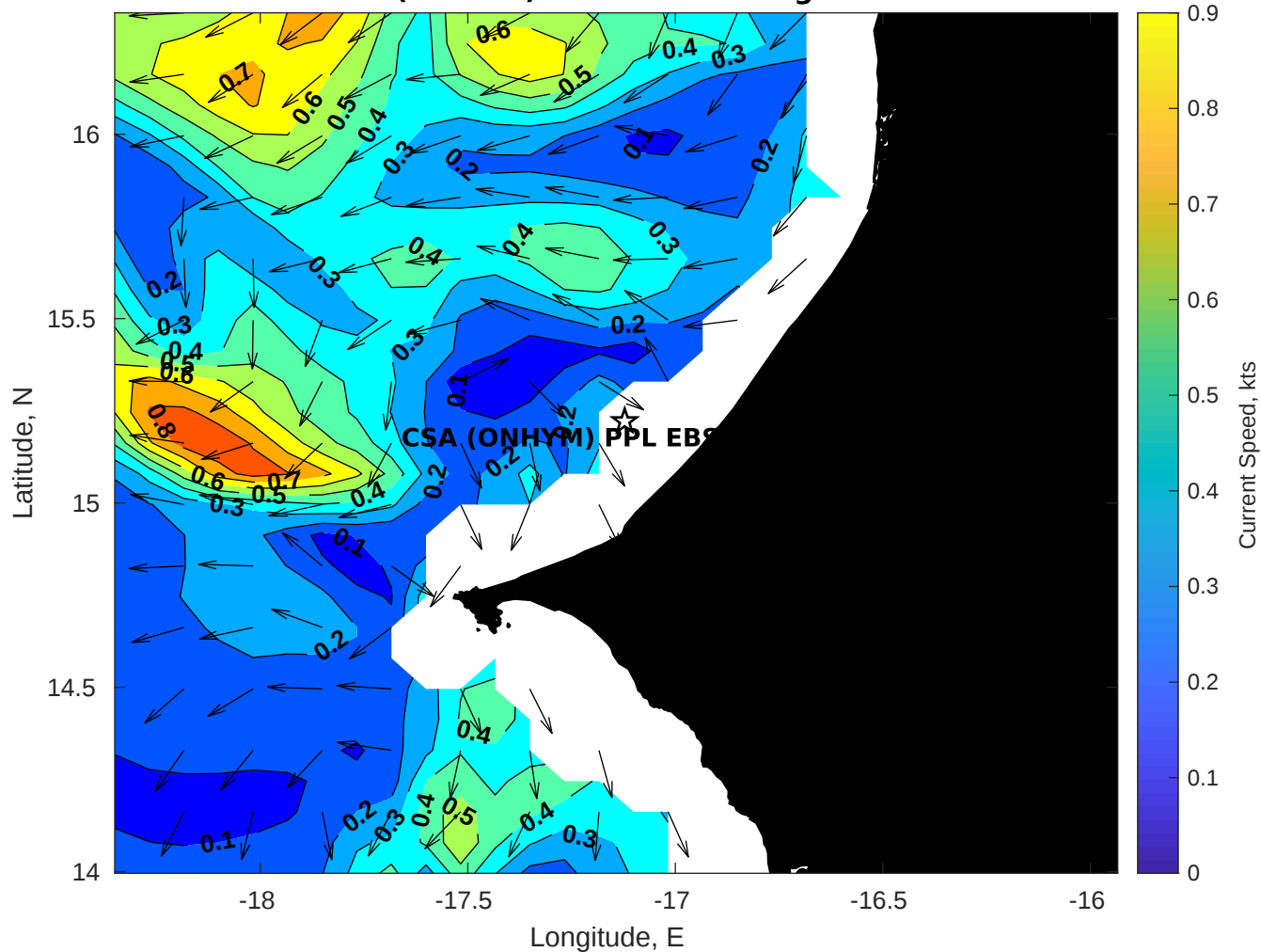
Surface Currents for CSA (ONHYM) PPL EBS - Senegal at 23-Dec-2025 00:00:00
