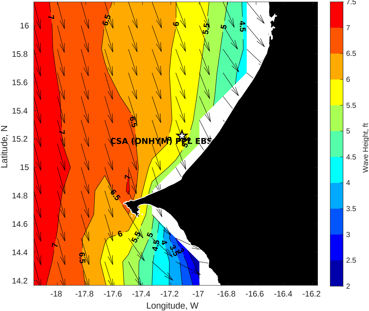
GFS Wave Height (ft) for CSA (ONHYM) PPL EBS - Senegal at 24-Dec-2025 09:00:00
