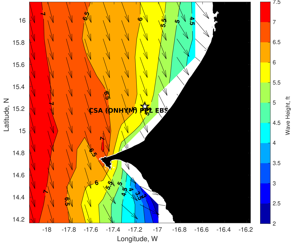
GFS Wave Height (ft) for CSA (ONHYM) PPL EBS - Senegal at 24-Dec-2025 09:00:00
