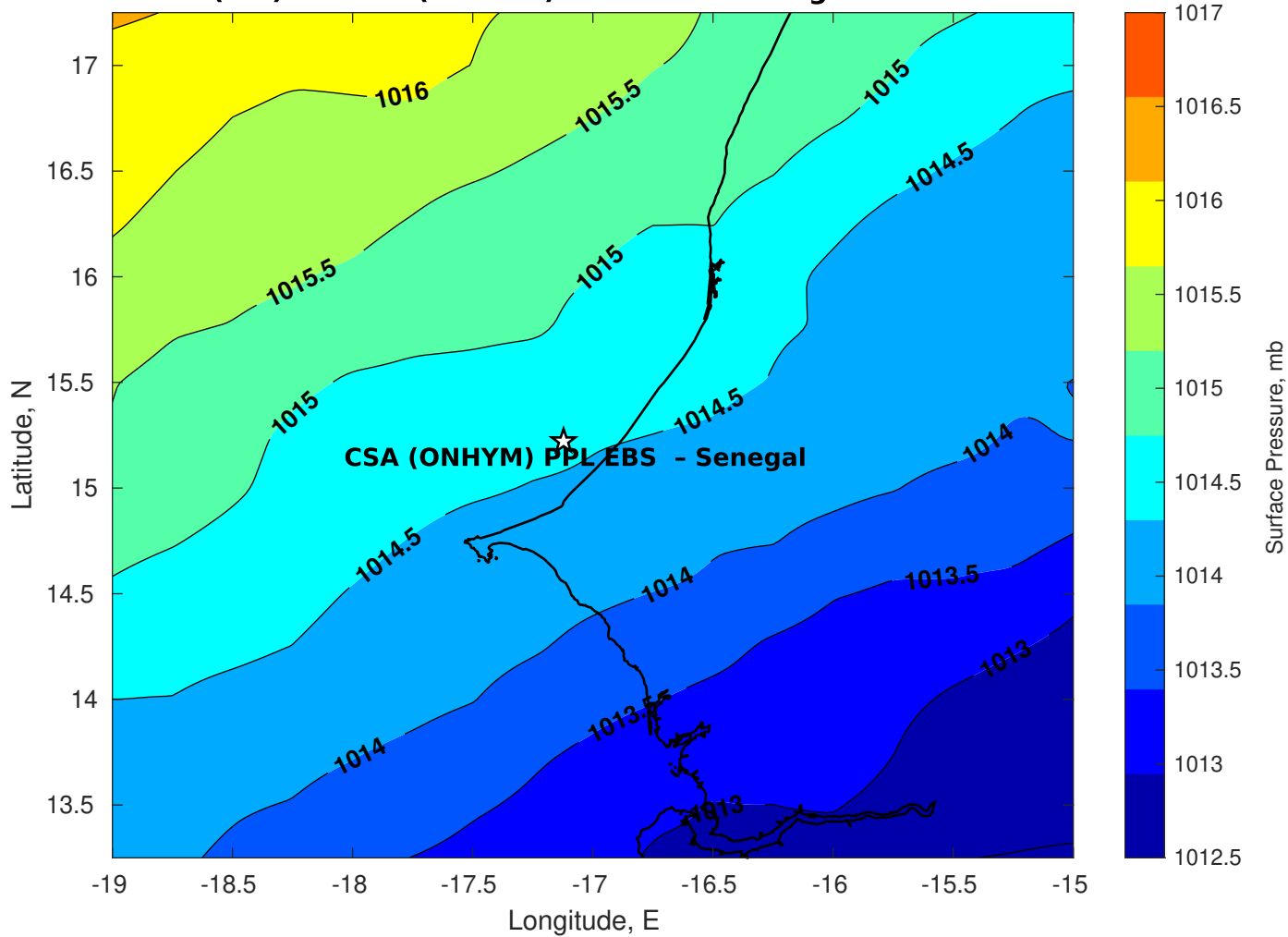
Surface Pressure (mb) for CSA (ONHYM) PPL EBS - Senegal at 26-Dec-2025 00:00:00
