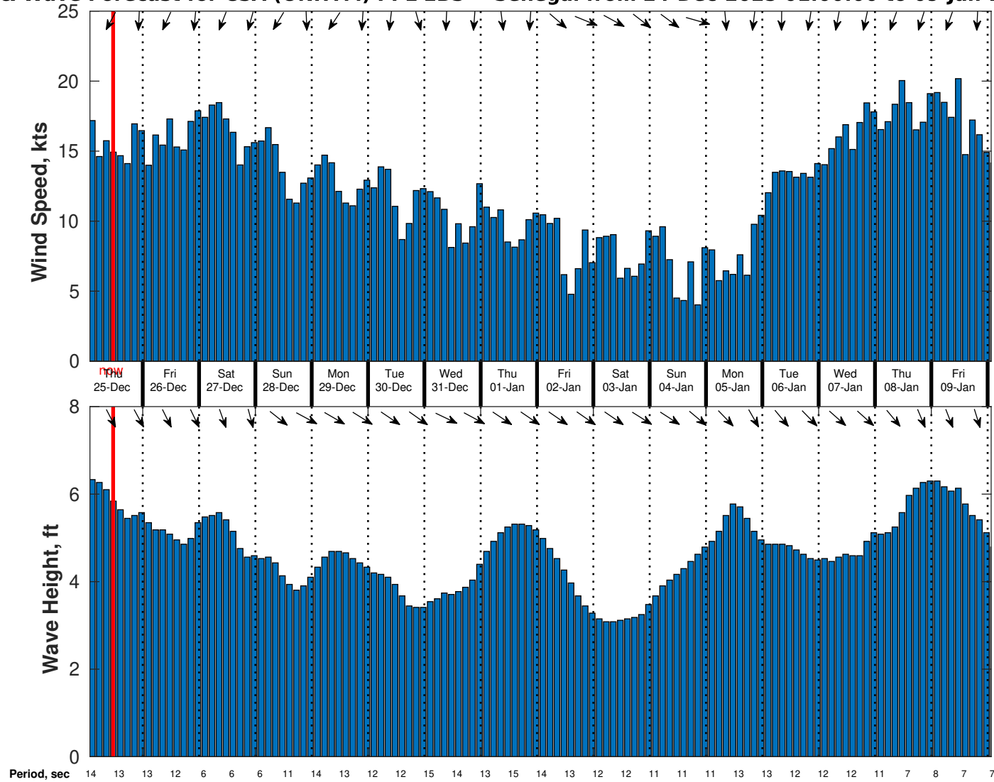
Wind & Wave Forecast for CSA (ONHYM) PPL EBS - Senegal from 24-Dec-2025 01:00:00 to 09-Jan-2026 01:00:00
