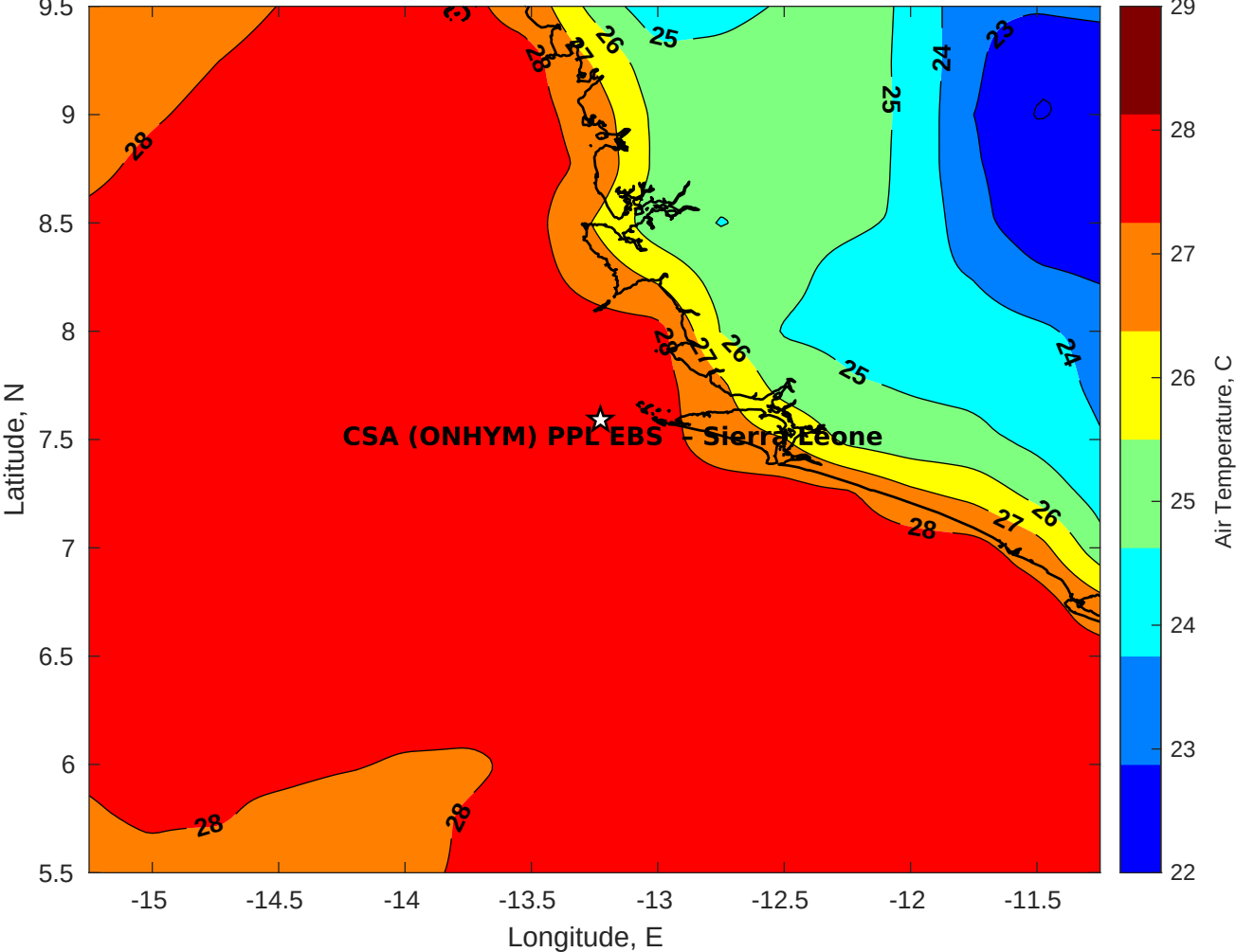
Air Temperature (C) for CSA (ONHYM) PPL EBS - Sierra Leone at 24-Dec-2025
