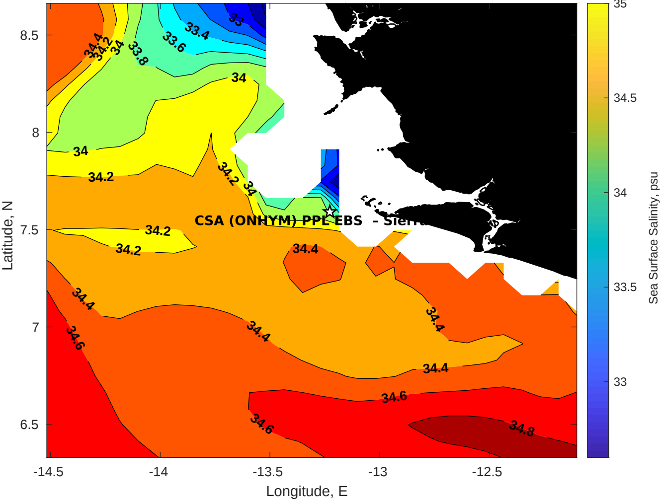
Surface Salinity for CSA (ONHYM) PPL EBS - Sierra Leone at 23-Dec-2025 00:00:00
