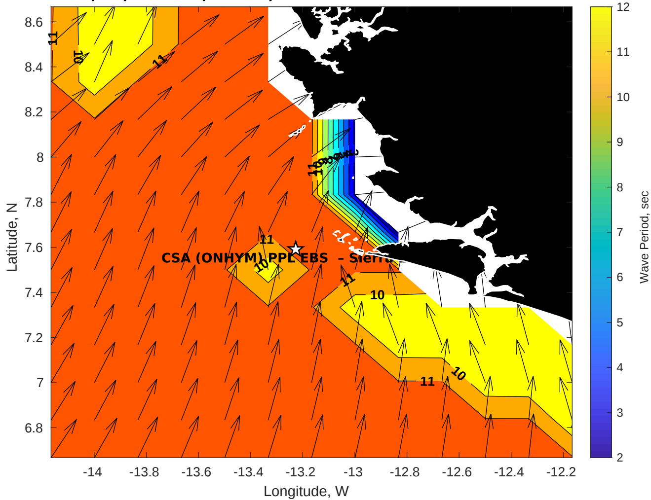
GFS Wave Period (sec) for CSA (ONHYM) PPL EBS - Sierra Leone at 24-Dec-2025 09:00:00
