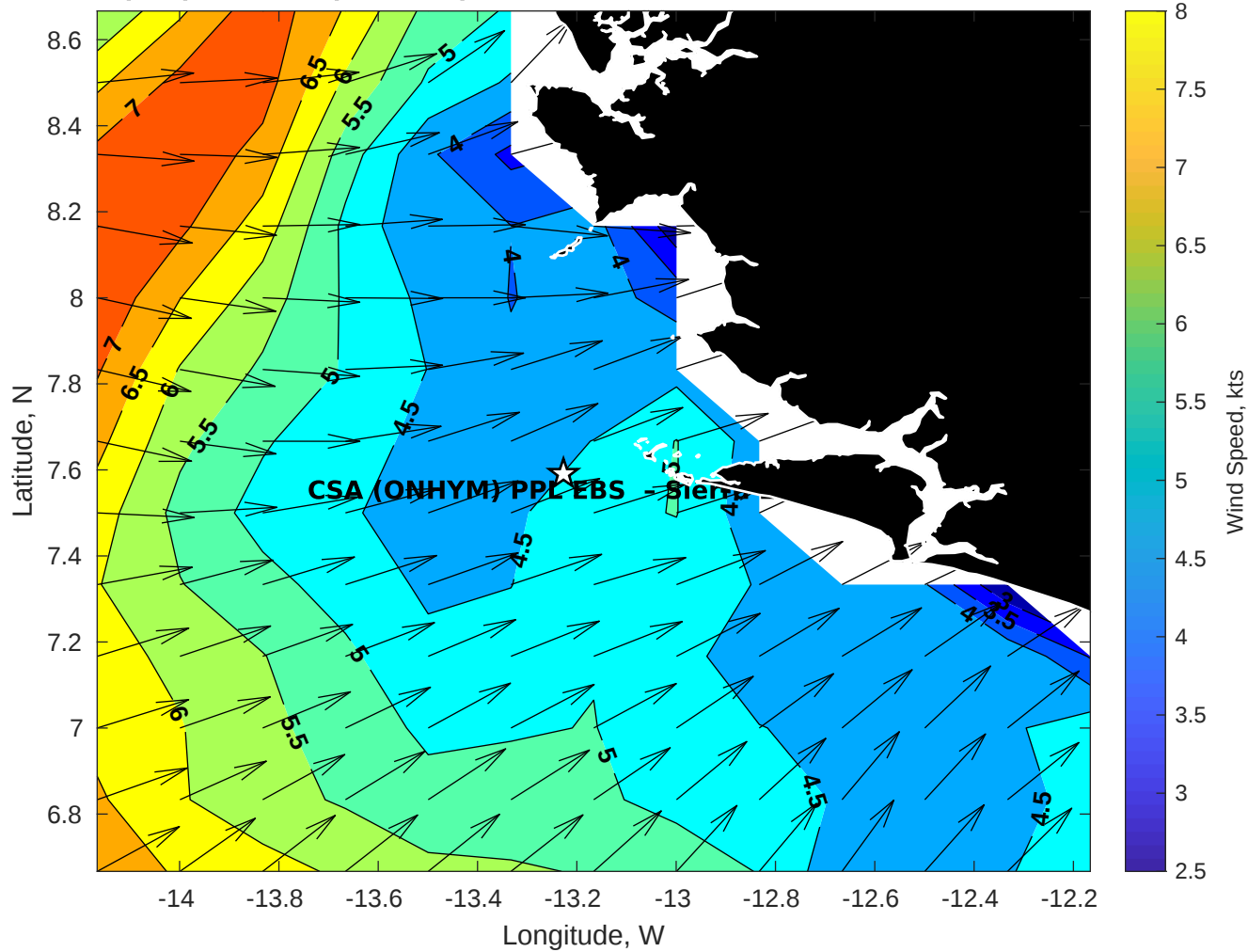
GFS Winds (kts) for CSA (ONHYM) PPL EBS - Sierra Leone at 24-Dec-2025 09:00:00
