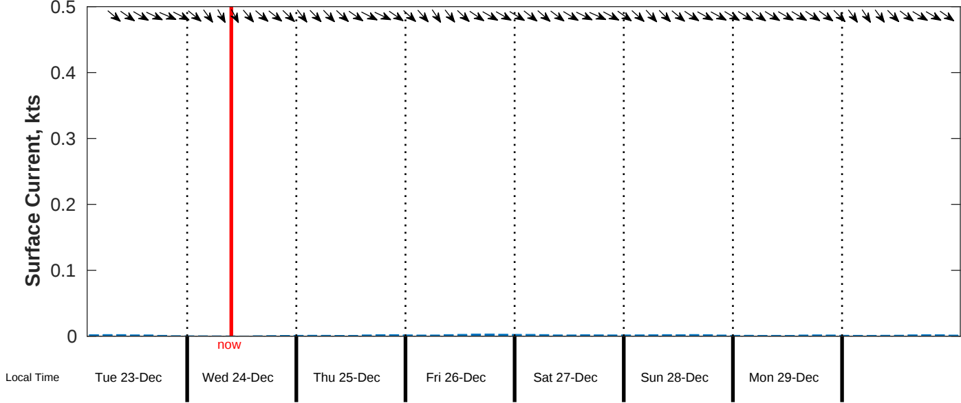
Surface Current Forecast for CSA (ONHYM) PPL EBS - Sierra Leone from 23-Dec-2025 00:00:00 to 31-Dec-2025 00:00:00
