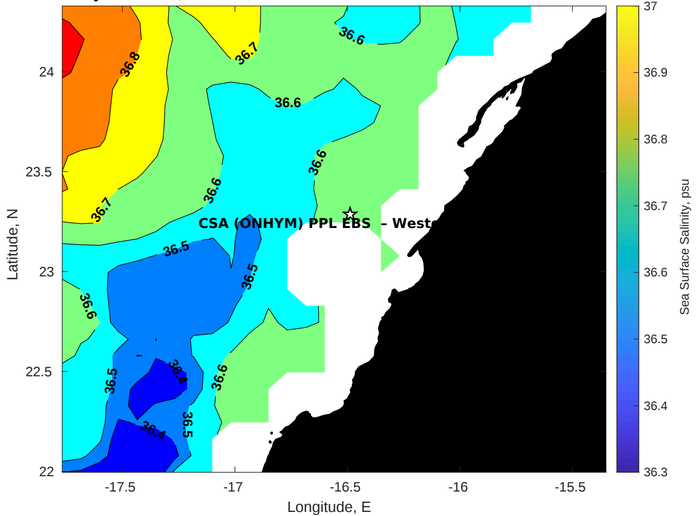
Surface Salinity for CSA (ONHYM) PPL EBS - Western Sahara at 23-Dec-2025 00:00:00
