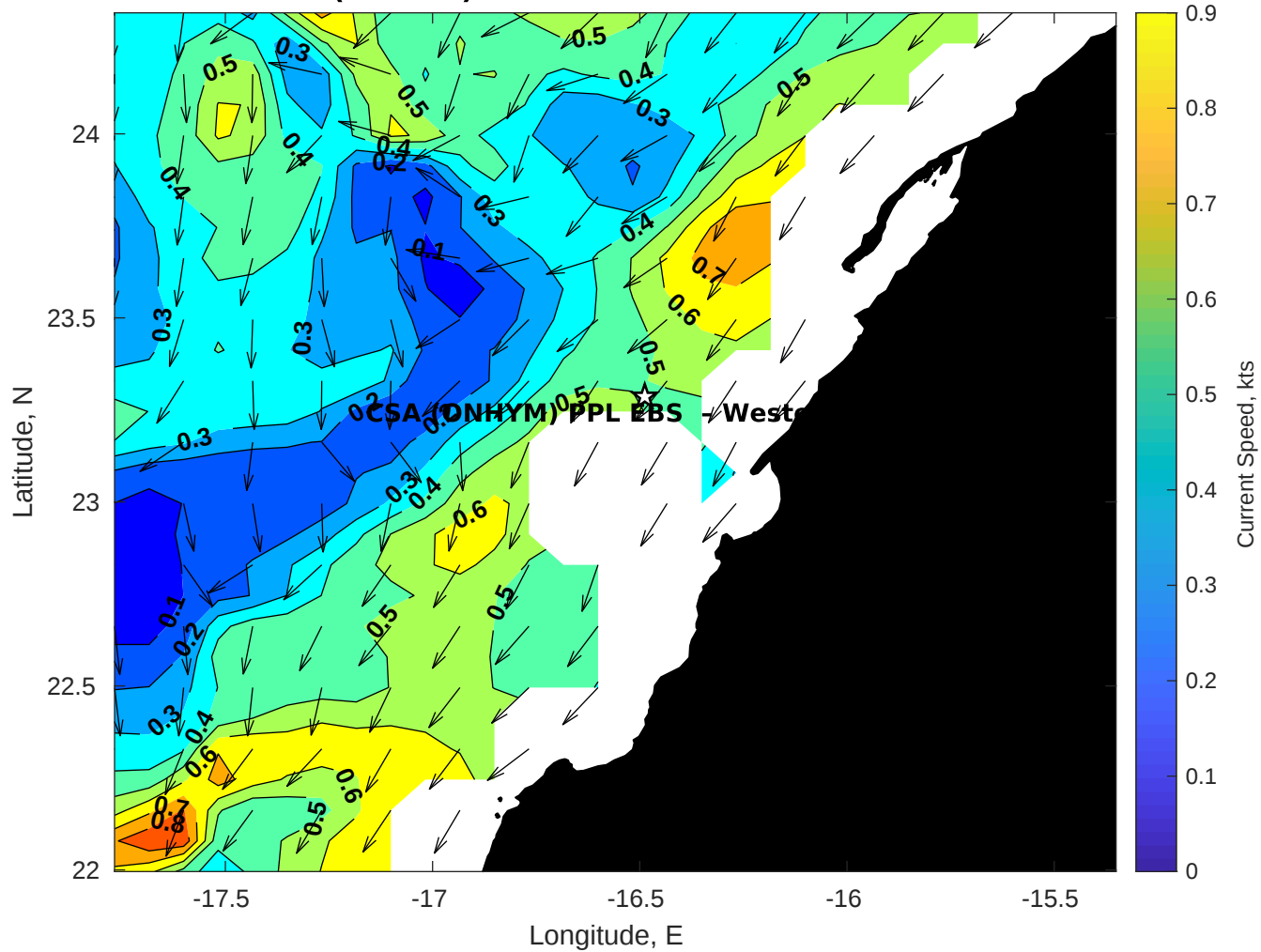
Surface Currents for CSA (ONHYM) PPL EBS - Western Sahara at 23-Dec-2025 00:00:00
