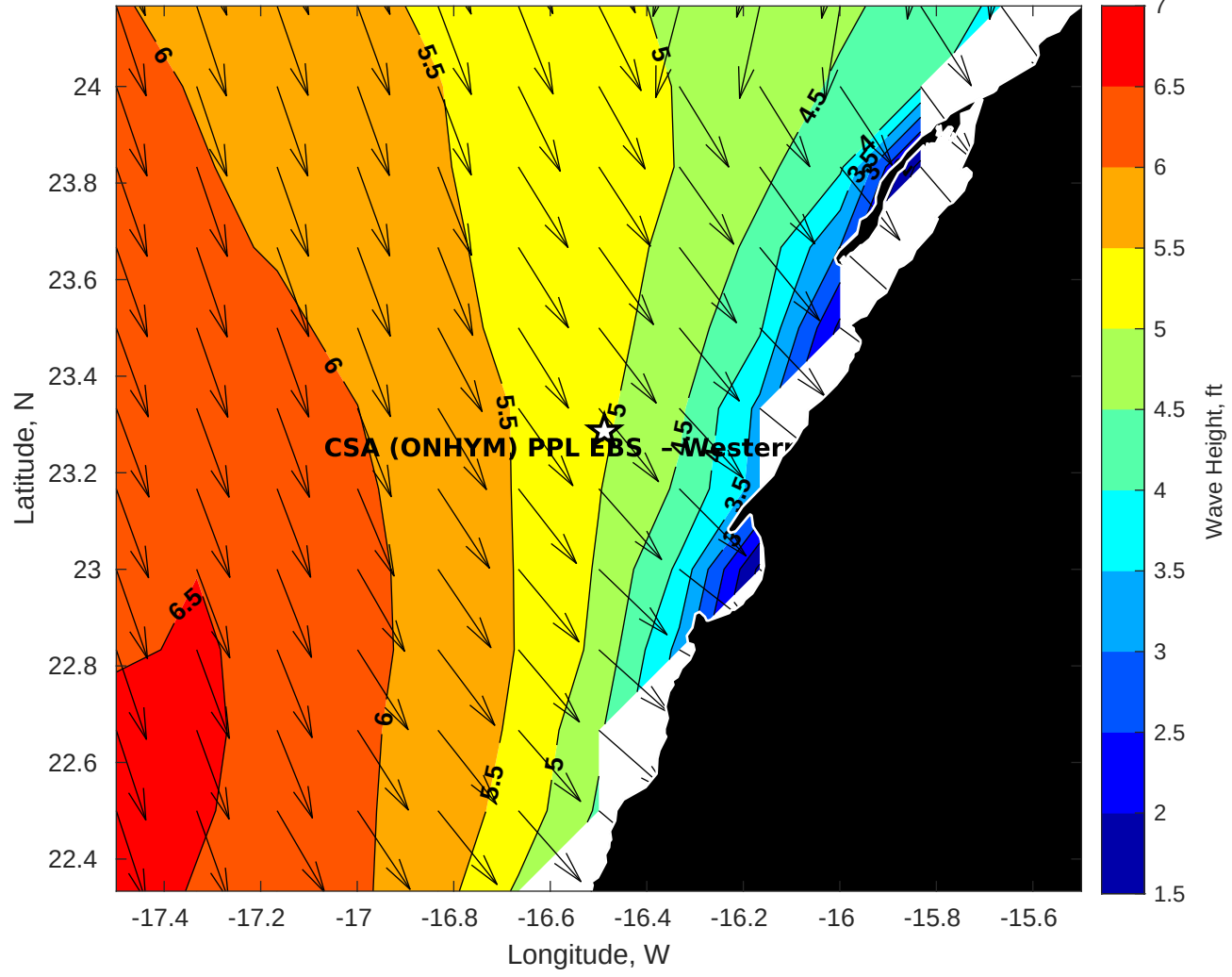
GFS Wave Height (ft) for CSA (ONHYM) PPL EBS - Western Sahara at 24-Dec-2025 09:00:00
