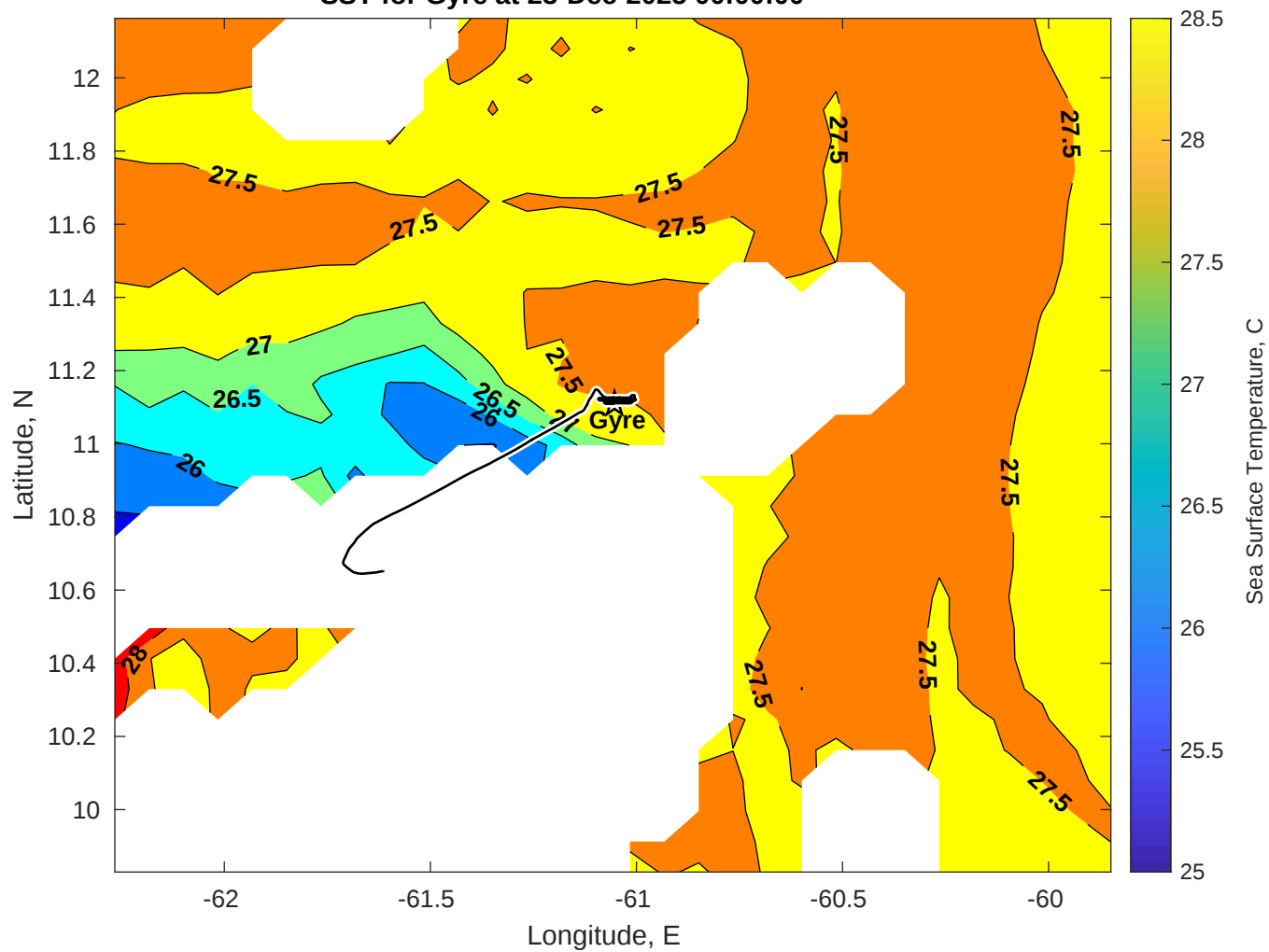
SST for Gyre at 23-Dec-2025 00:00:00
