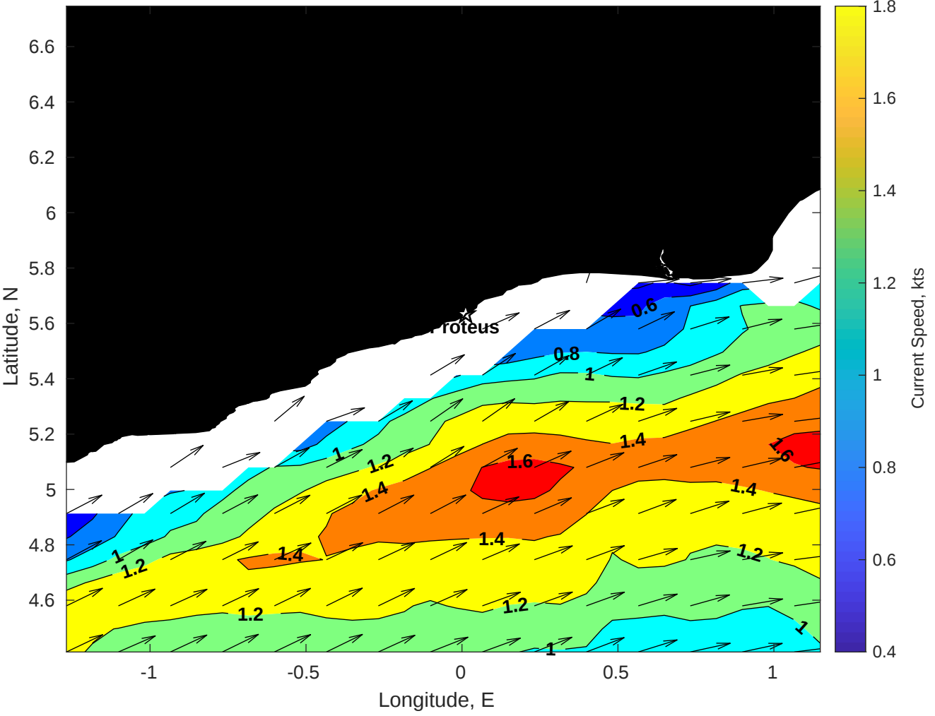
Surface Currents for Proteus at 23-Dec-2025 00:00:00
