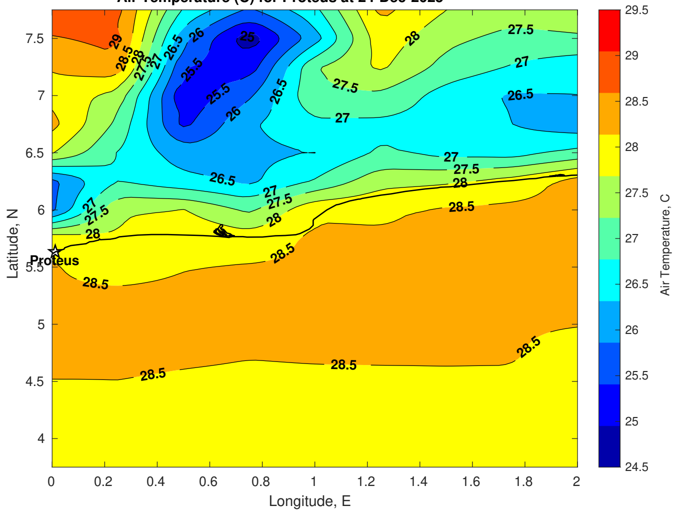
Air Temperature (C) for Proteus at 24-Dec-2025
