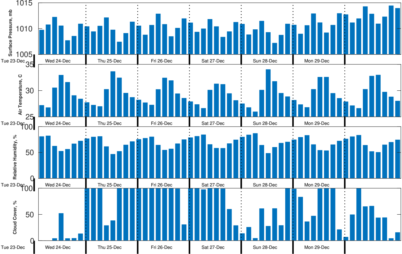
Met Forecast for Proteus from 24-Dec-2025 00:00:00 to 31-Dec-2025 00:00:00
