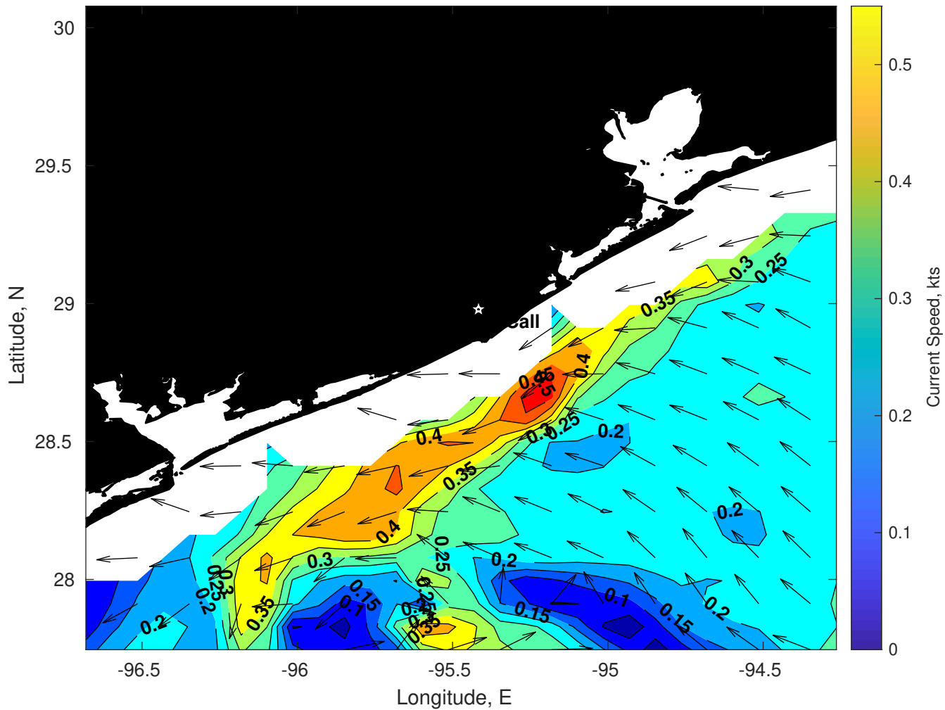
Surface Currents for Brooks McCall at 24-Dec-2025 00:00:00
