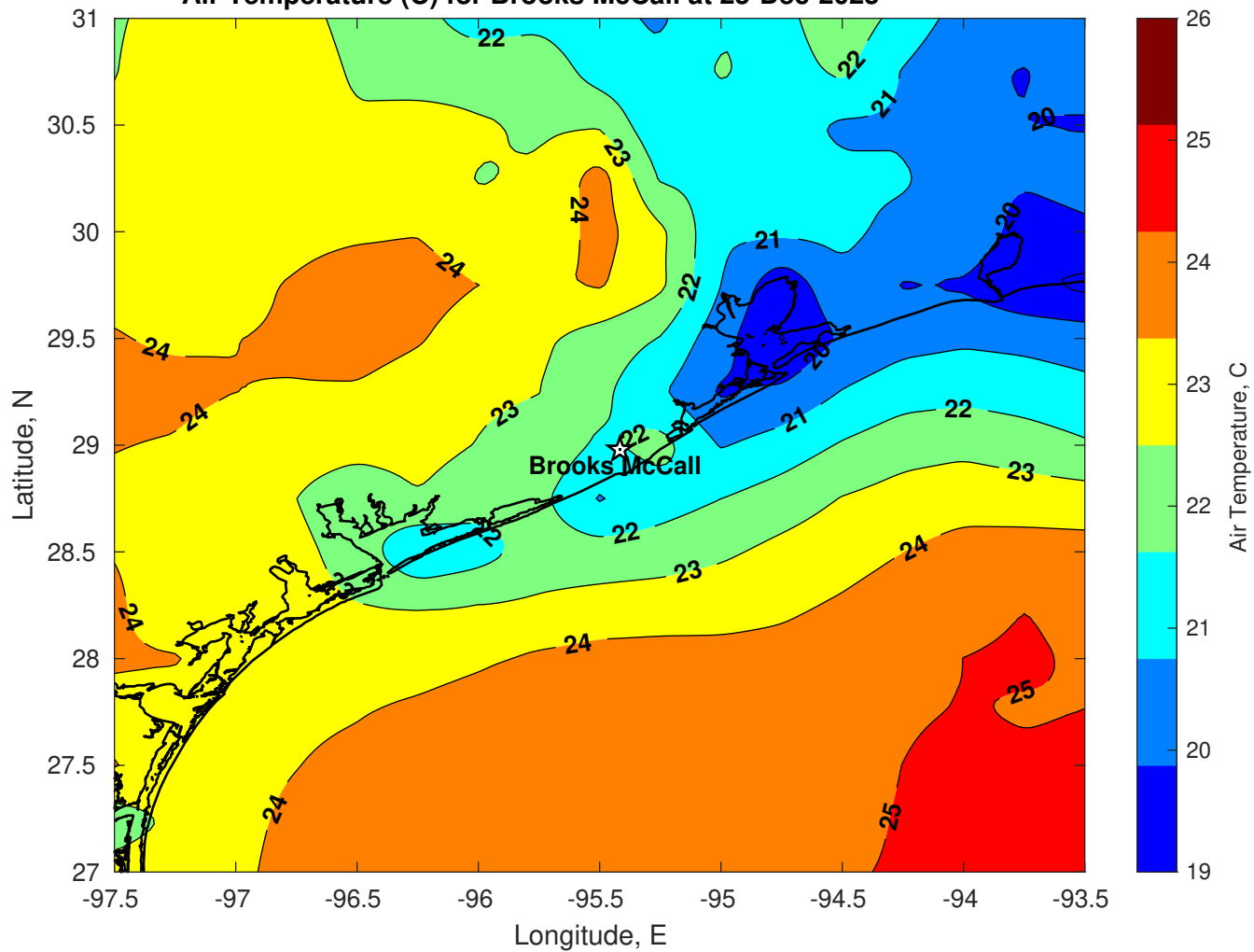
Air Temperature (C) for Brooks McCall at 25-Dec-2025
