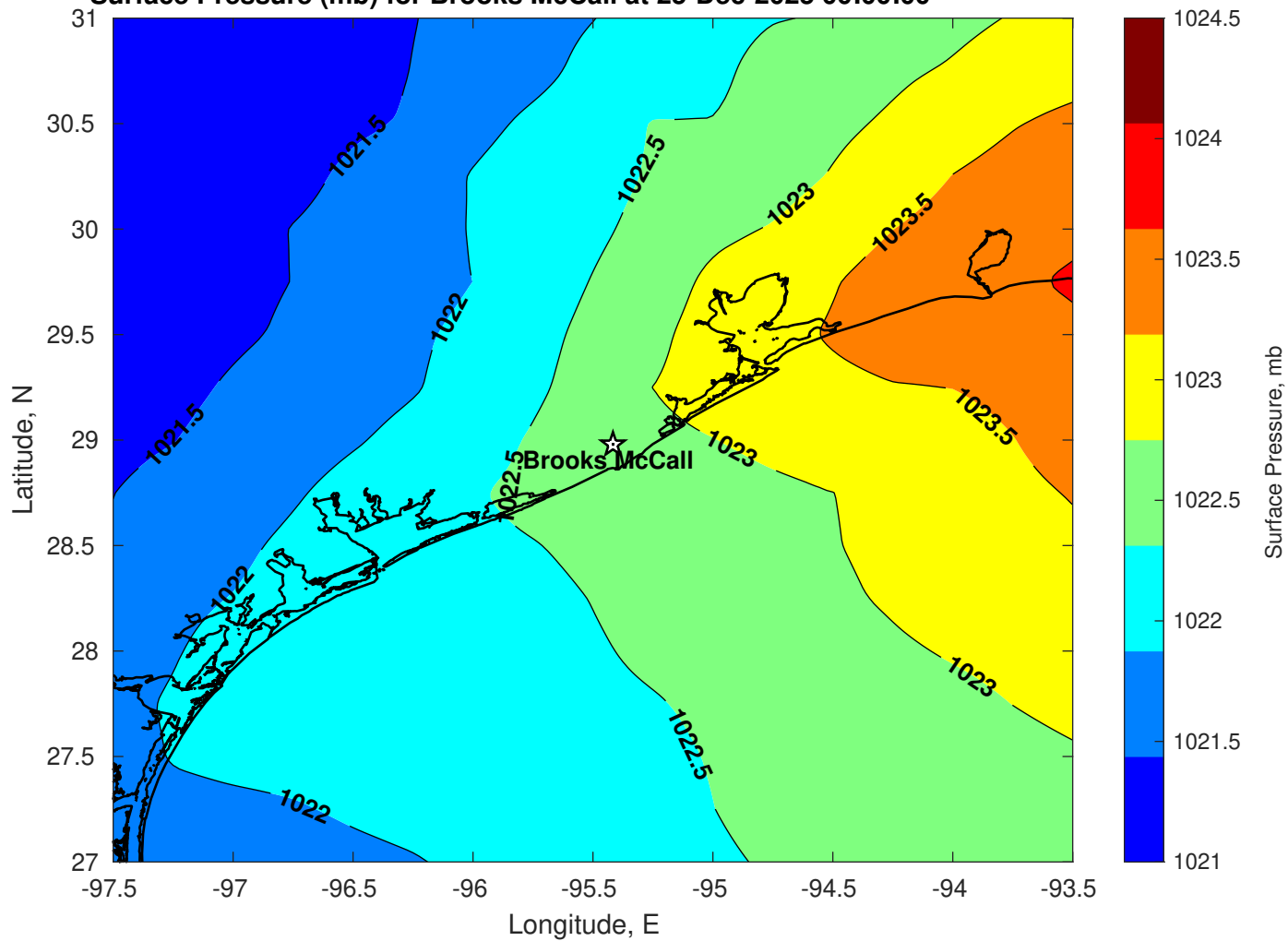
Surface Pressure (mb) for Brooks McCall at 25-Dec-2025 00:00:00
