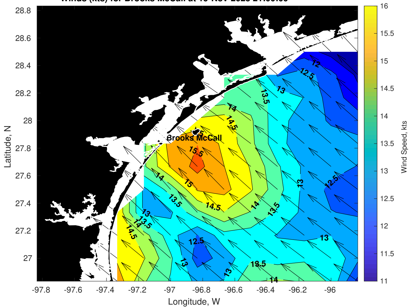
Winds (kts) for Brooks McCall at 19-Nov-2025 21:00:00
