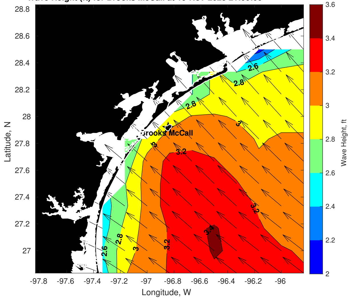
Wave Height (ft) for Brooks McCall at 19-Nov-2025 21:00:00
