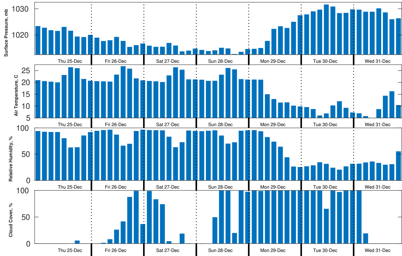
Met Forecast for Brooks McCall from 25-Dec-2025 00:00:00 to 01-Jan-2026 00:00:00
