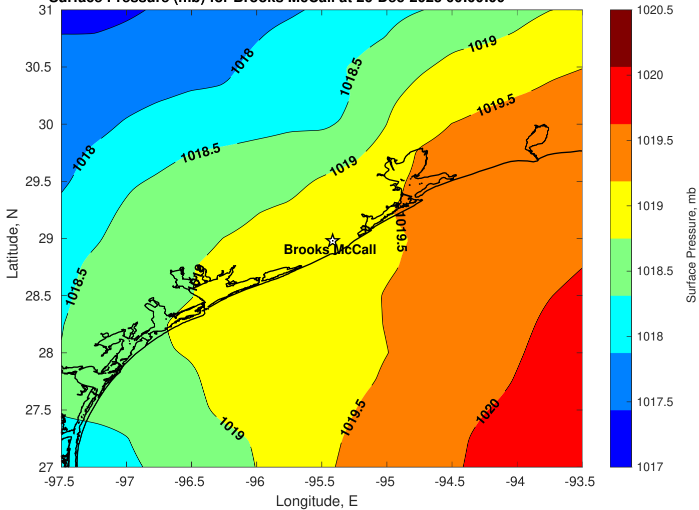
Surface Pressure (mb) for Brooks McCall at 26-Dec-2025 00:00:00
