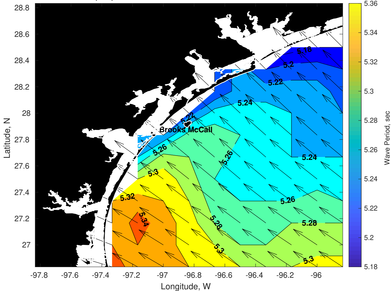
Wave Period (sec) for Brooks McCall at 19-Nov-2025 21:00:00
