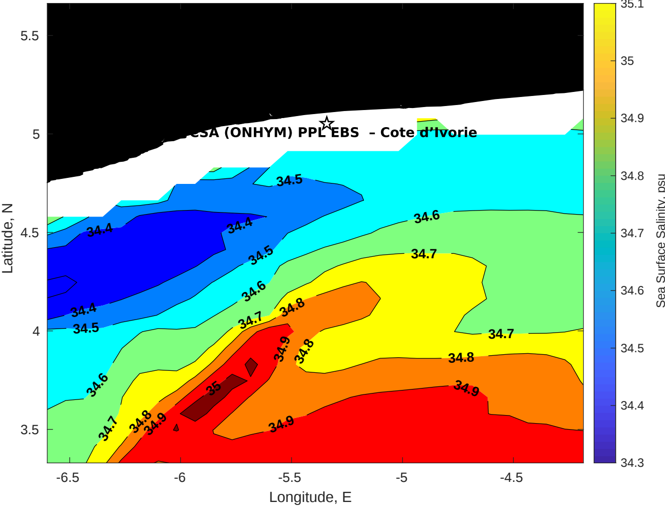
Surface Salinity for CSA (ONHYM) PPL EBS - Cote d'Ivoire at 24-Dec-2025 00:00:00
