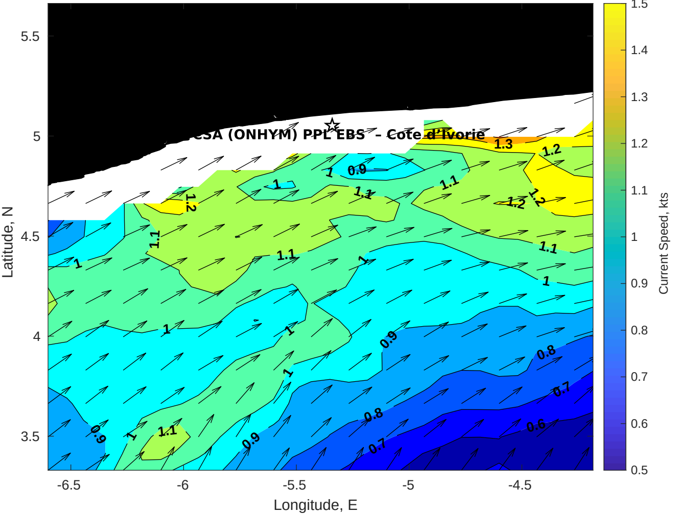
Surface Currents for CSA (ONHYM) PPL EBS - Cote d'Ivoire at 24-Dec-2025 00:00:00
