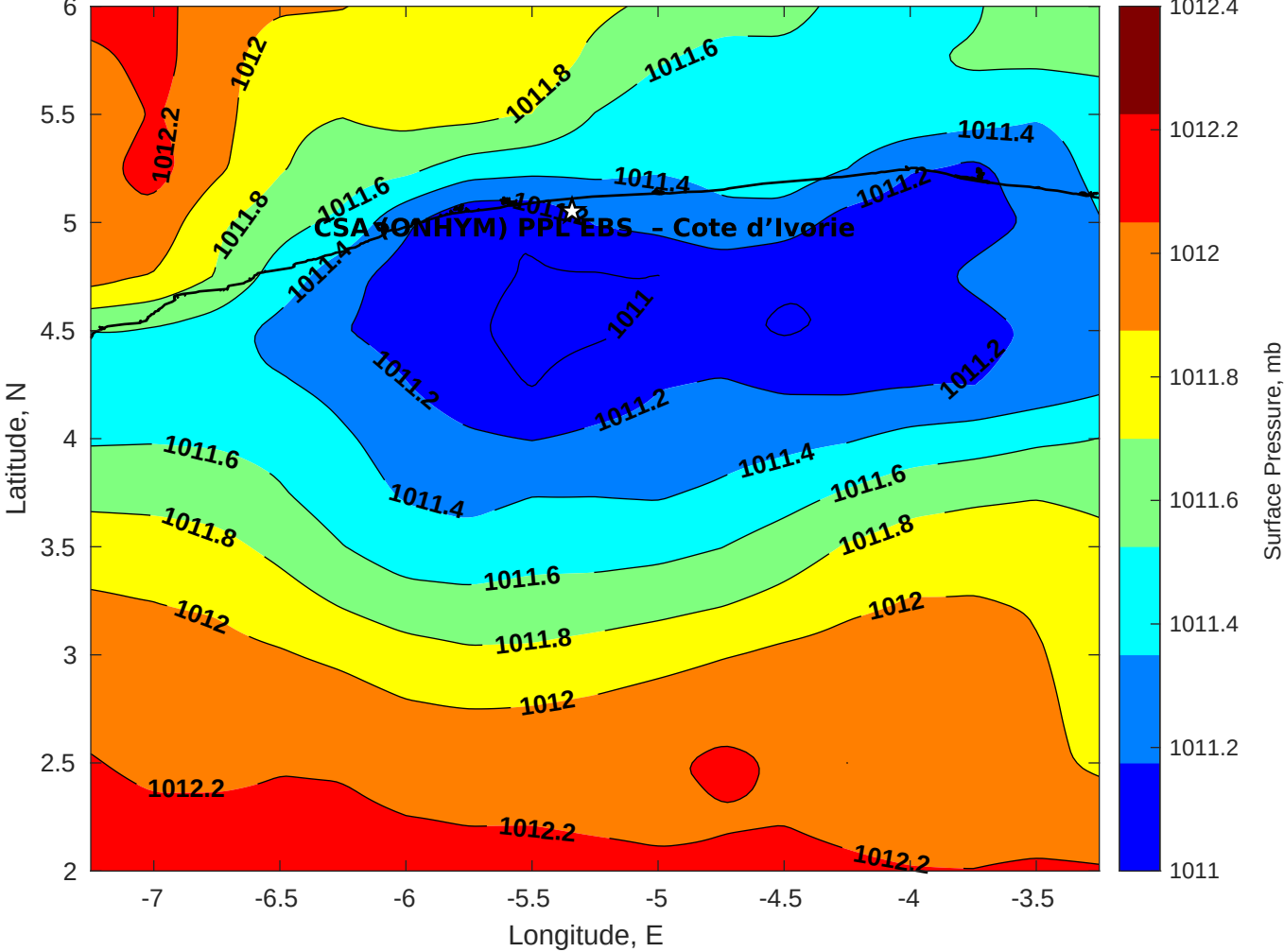
Surface Pressure (mb) for CSA (ONHYM) PPL EBS - Cote d'Ivoire at 26-Dec-2025 00:00:00
