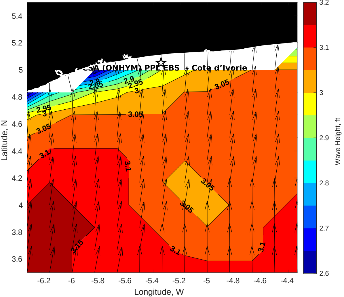
GFS Wave Height (ft) for CSA (ONHYM) PPL EBS - Cote d'Ivoire at 25-Dec-2025 09:00:00
