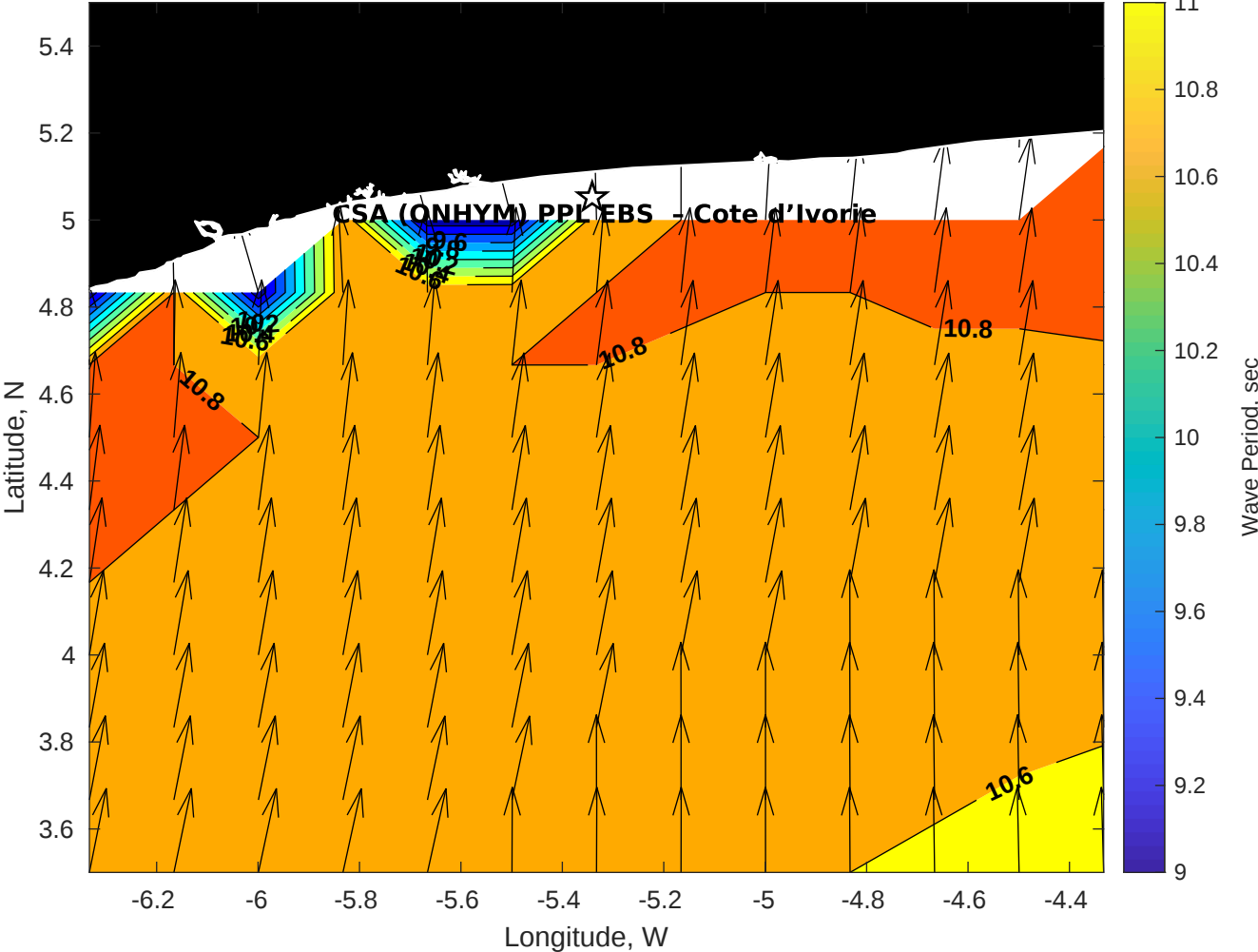
GFS Wave Period (sec) for CSA (ONHYM) PPL EBS - Cote d'Ivoire at 25-Dec-2025 09:00:00
