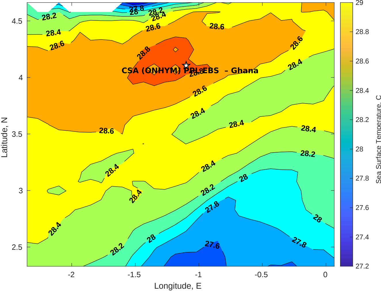
SST for CSA (ONHYM) PPL EBS - Ghana at 24-Dec-2025 00:00:00
