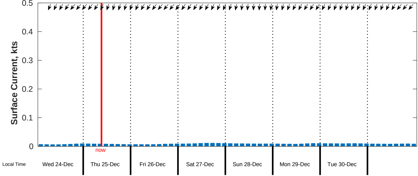
Surface Current Forecast for CSA (ONHYM) PPL EBS - Ghana from 24-Dec-2025 00:00:00 to 01-Jan-2026 00:00:00
