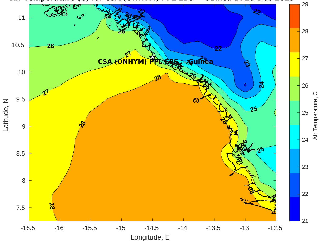
Air Temperature (C) for CSA (ONHYM) PPL EBS - Guinea at 25-Dec-2025
