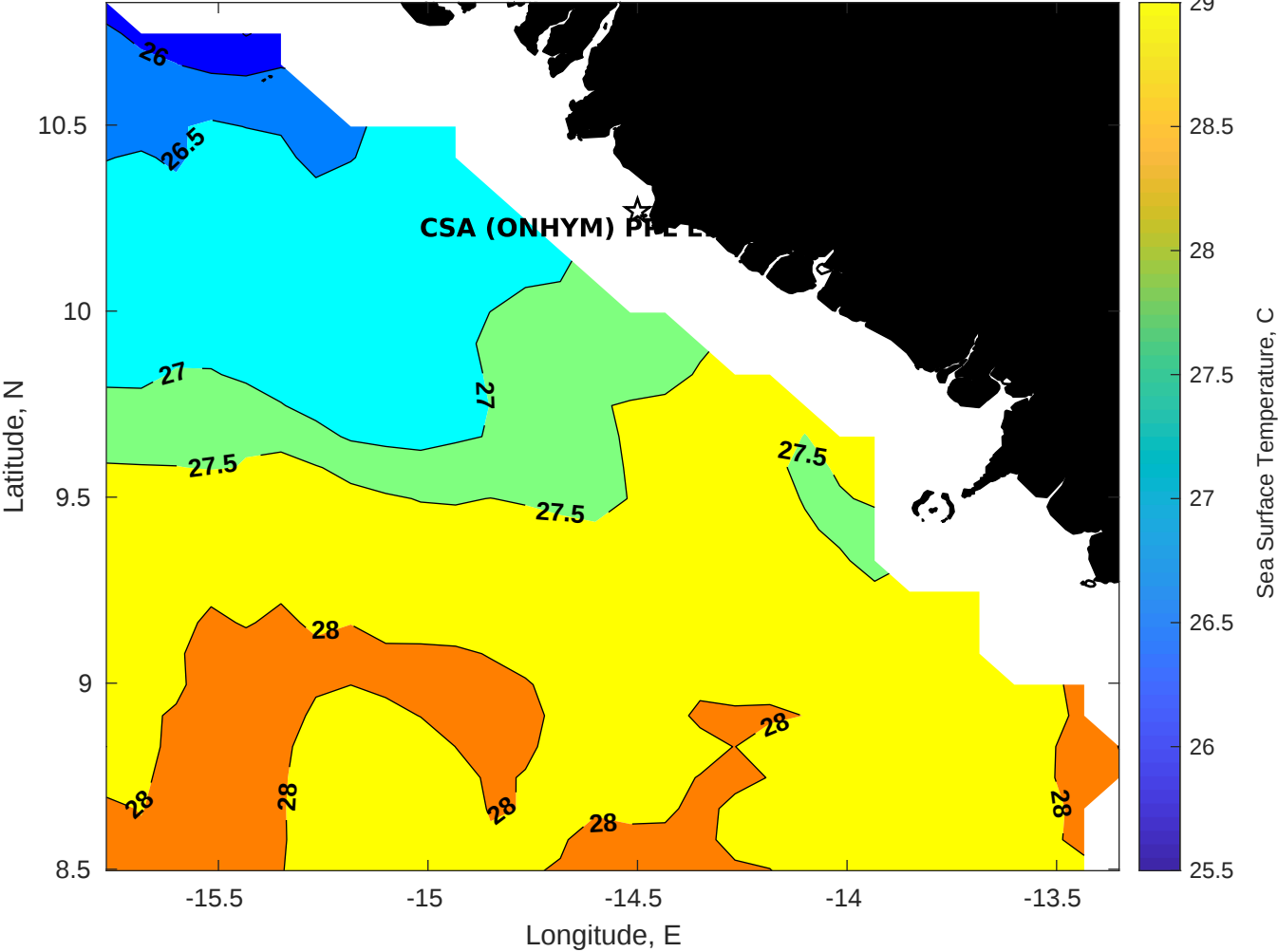
SST for CSA (ONHYM) PPL EBS - Guinea at 24-Dec-2025 00:00:00
