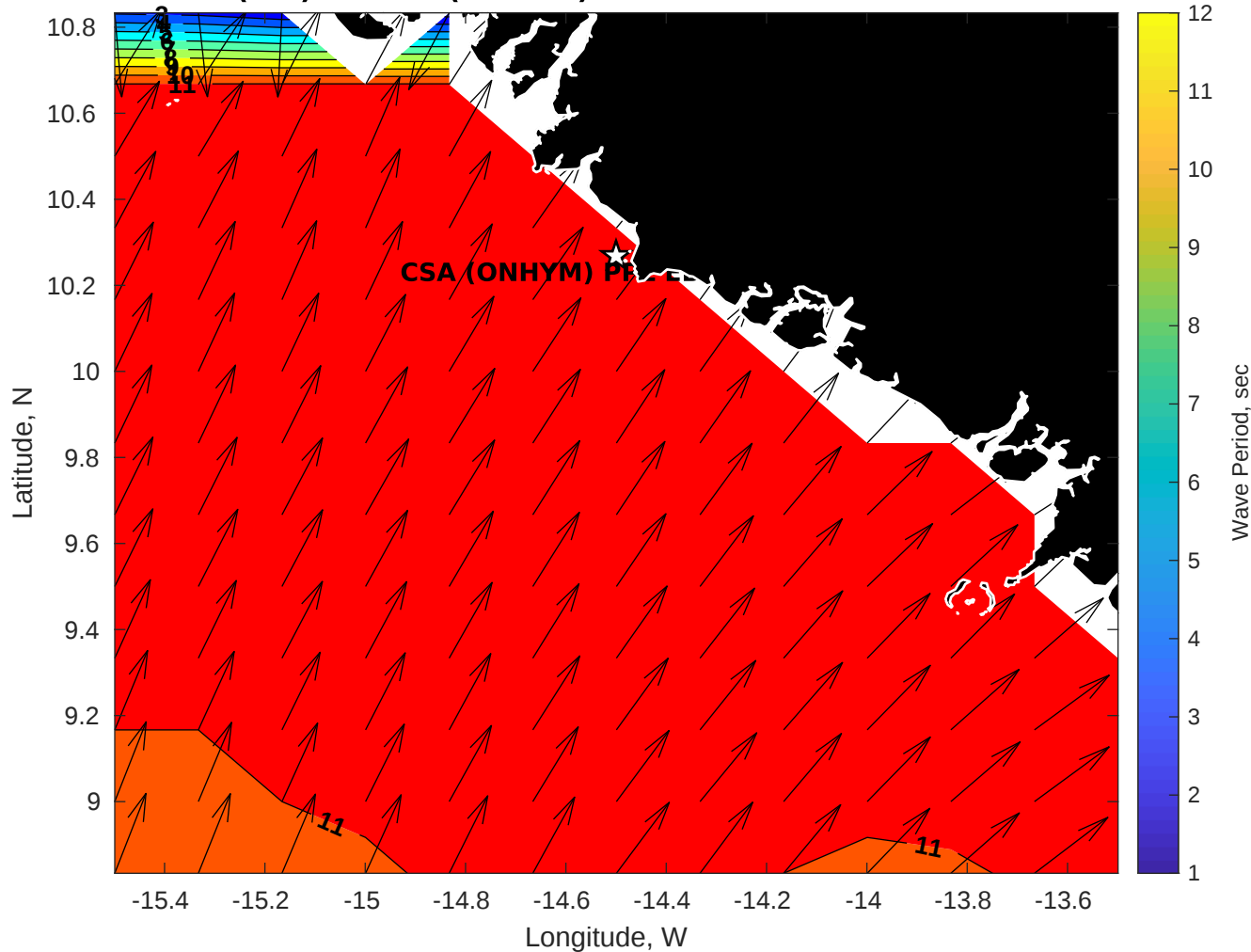
GFS Wave Period (sec) for CSA (ONHYM) PPL EBS - Guinea at 25-Dec-2025 09:00:00
