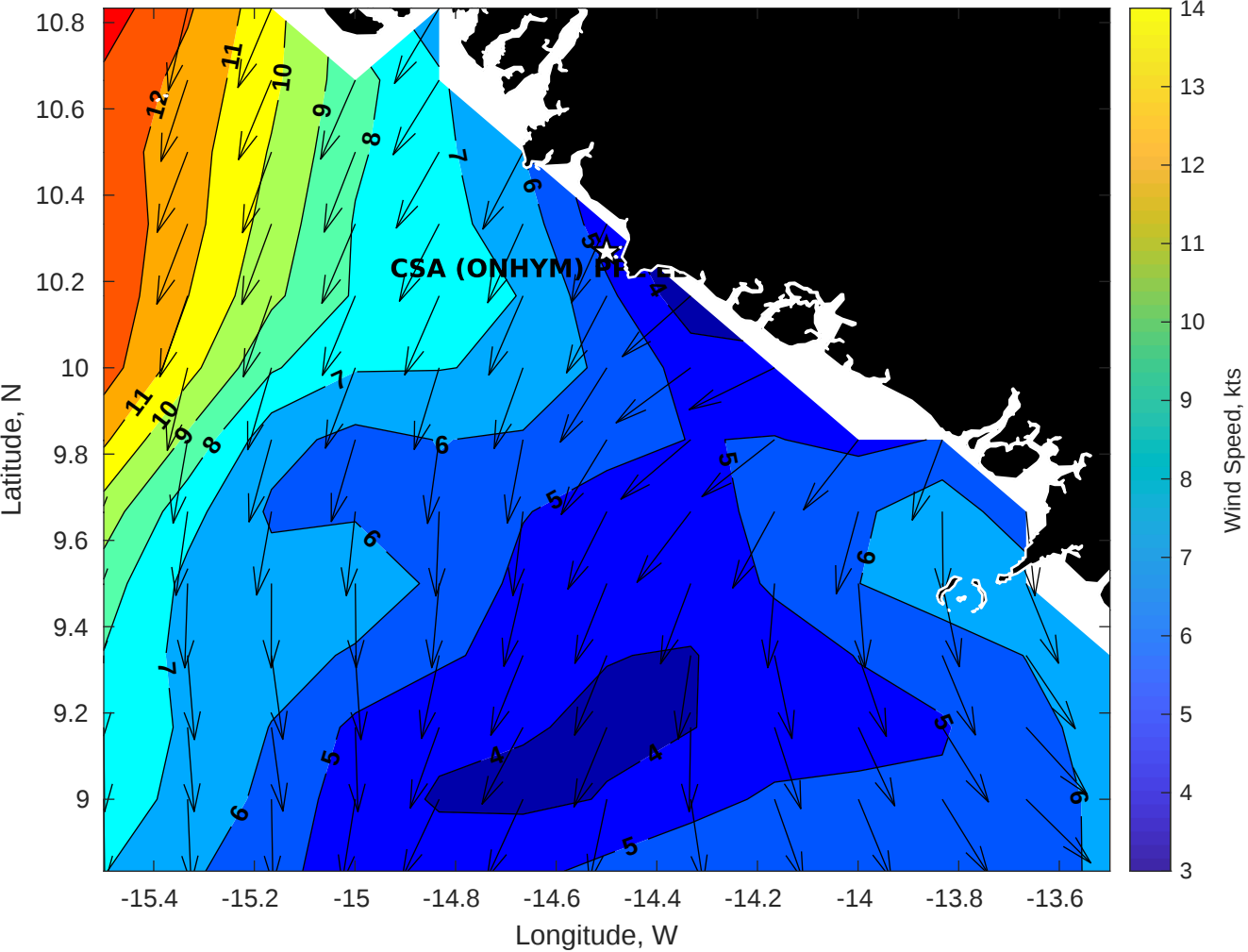
GFS Winds (kts) for CSA (ONHYM) PPL EBS - Guinea at 25-Dec-2025 09:00:00
