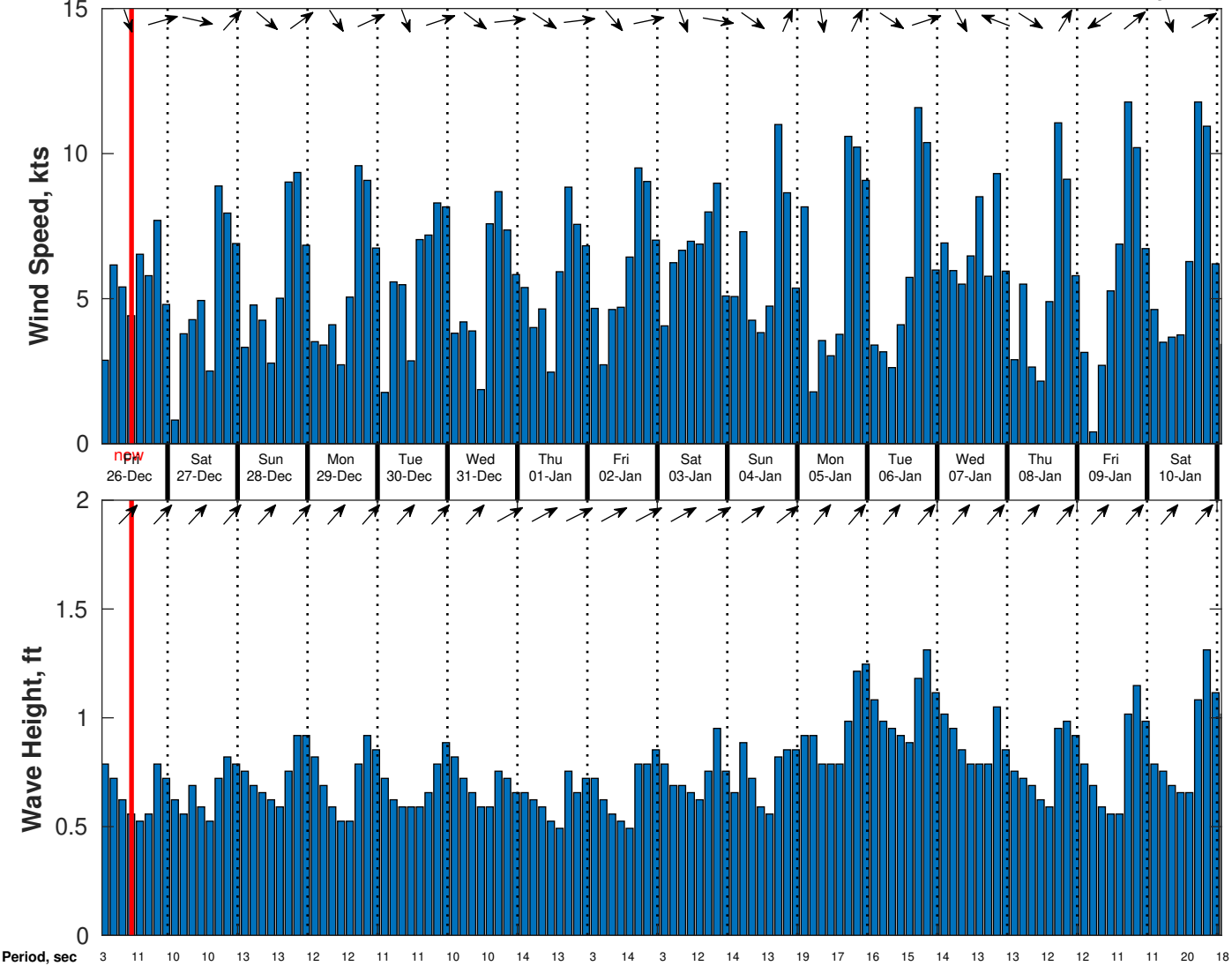
Wind & Wave Forecast for CSA (ONHYM) PPL EBS - Guinea from 25-Dec-2025 01:00:00 to 10-Jan-2026 01:00:00
