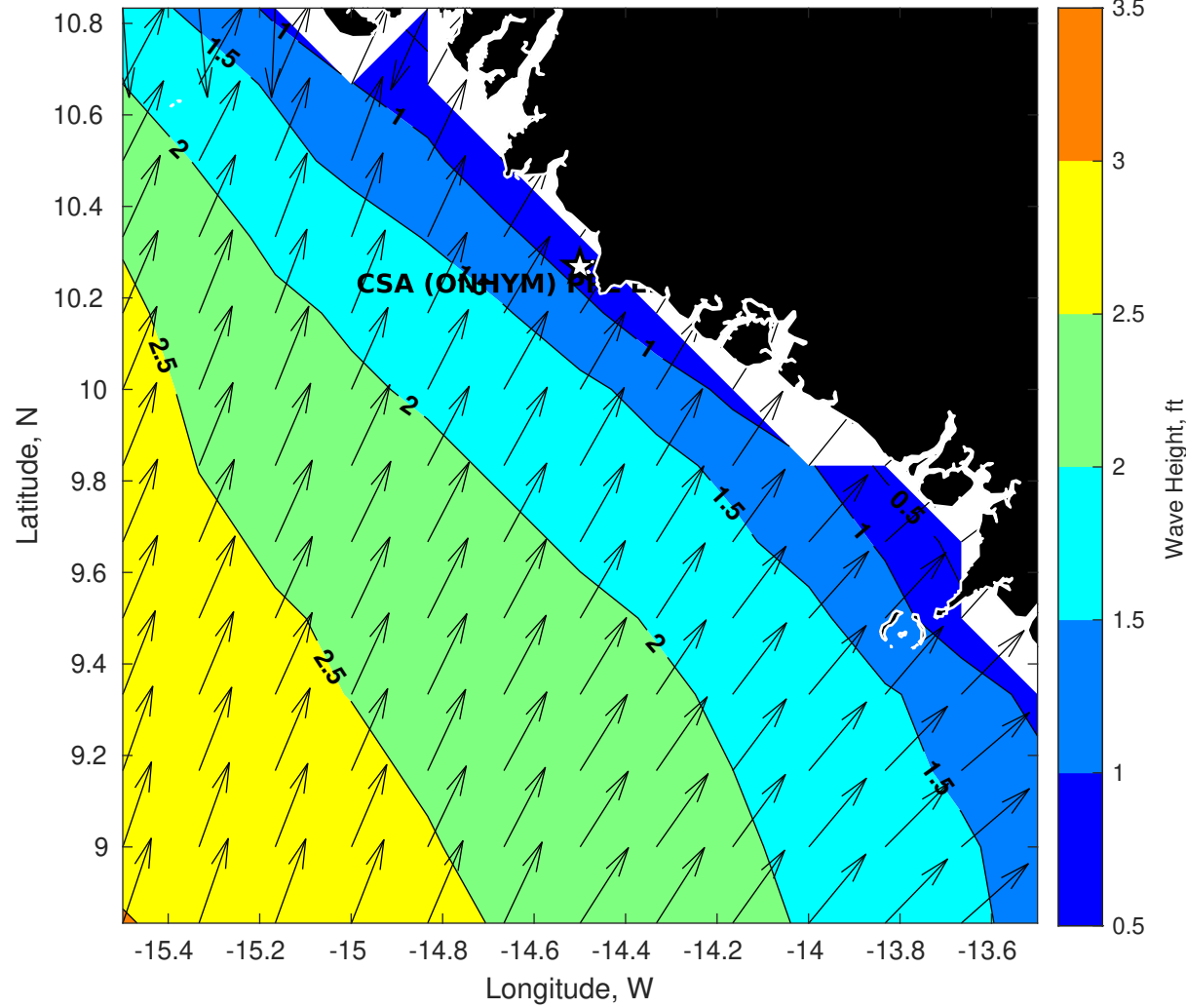
GFS Wave Height (ft) for CSA (ONHYM) PPL EBS - Guinea at 25-Dec-2025 09:00:00
