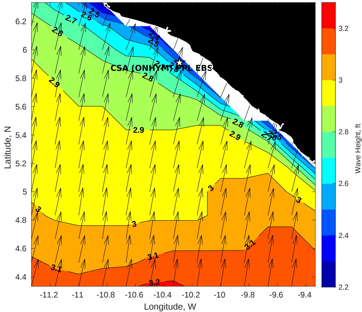
GFS Wave Height (ft) for CSA (ONHYM) PPL EBS - Liberia at 25-Dec-2025 09:00:00
