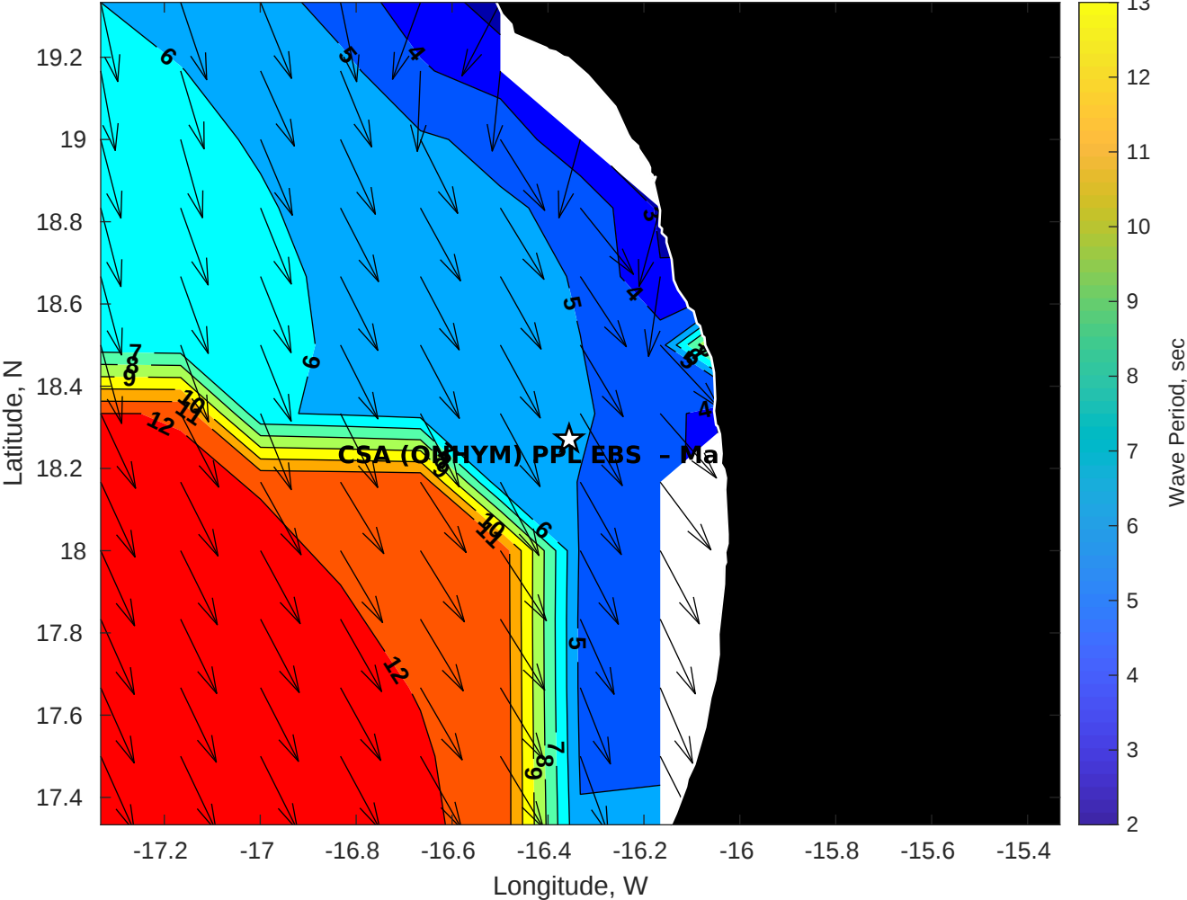
GFS Wave Period (sec) for CSA (ONHYM) PPL EBS - Mauritania at 25-Dec-2025 09:00:00
