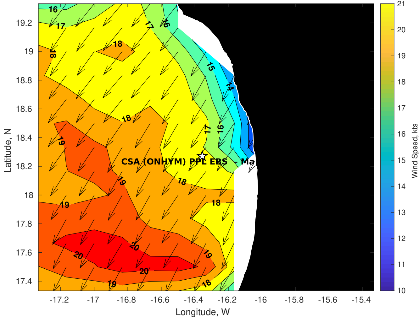
GFS Winds (kts) for CSA (ONHYM) PPL EBS - Mauritania at 25-Dec-2025 09:00:00
