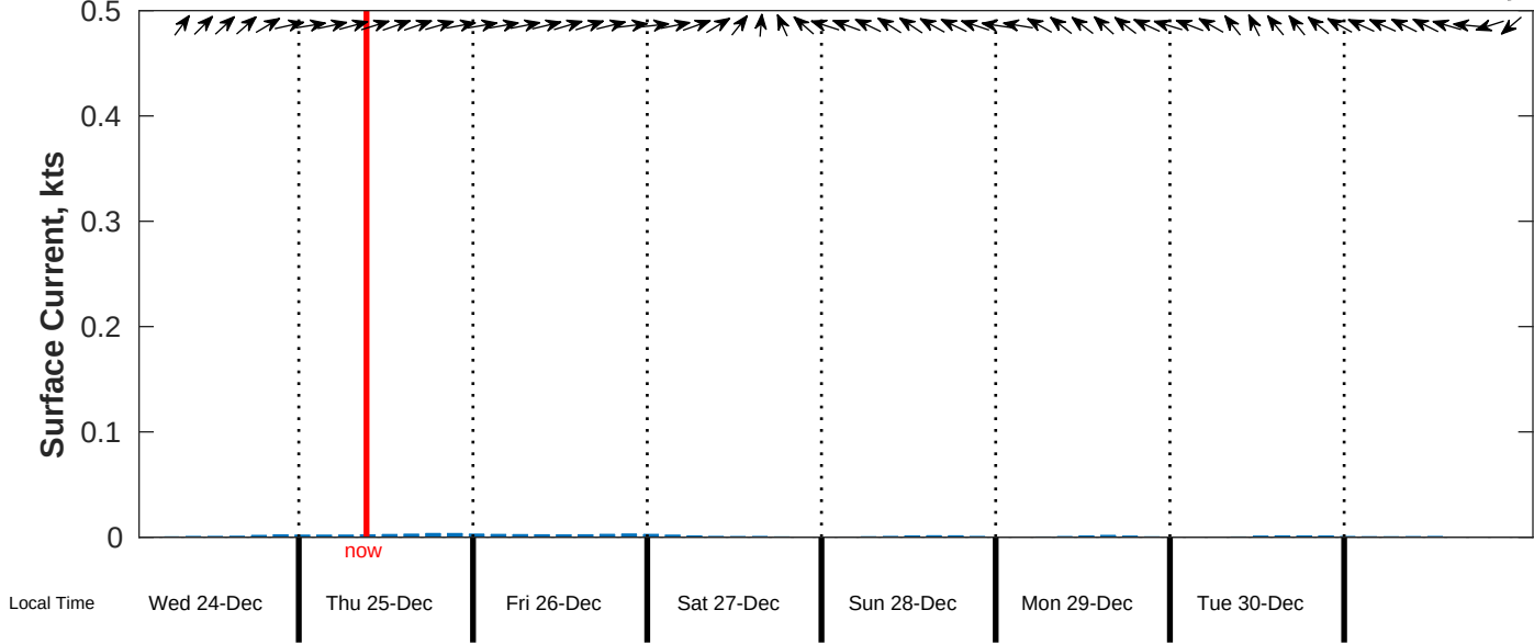
Surface Current Forecast for CSA (ONHYM) PPL EBS - Mauritania from 24-Dec-2025 00:00:00 to 01-Jan-2026 00:00:00
