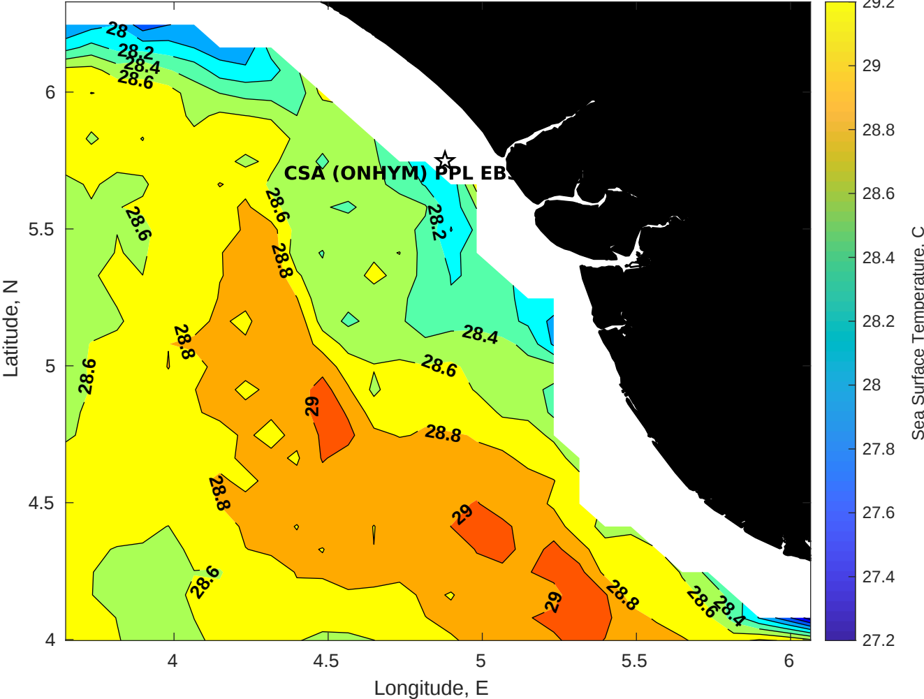
SST for CSA (ONHYM) PPL EBS - Nigeria at 24-Dec-2025 00:00:00
