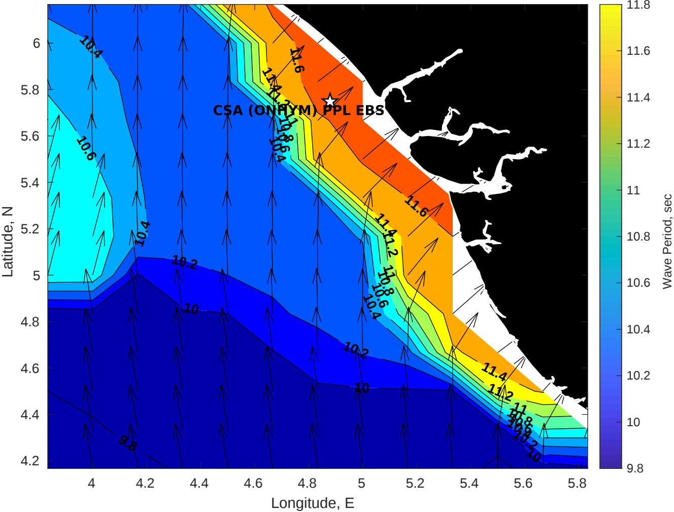
GFS Wave Period (sec) for CSA (ONHYM) PPL EBS - Nigeria at 25-Dec-2025 09:00:00
