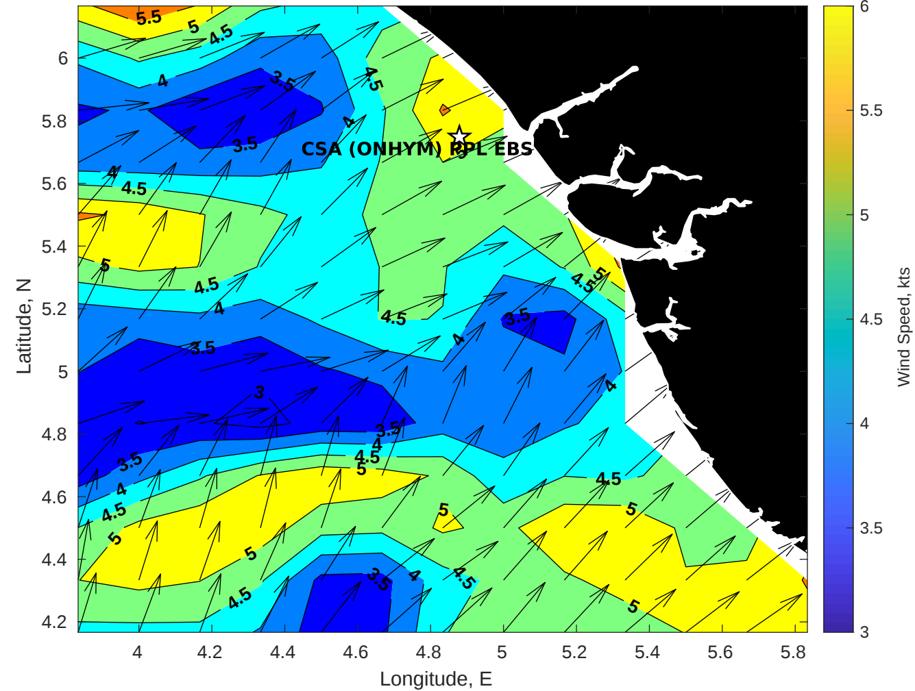
GFS Winds (kts) for CSA (ONHYM) PPL EBS - Nigeria at 25-Dec-2025 09:00:00
