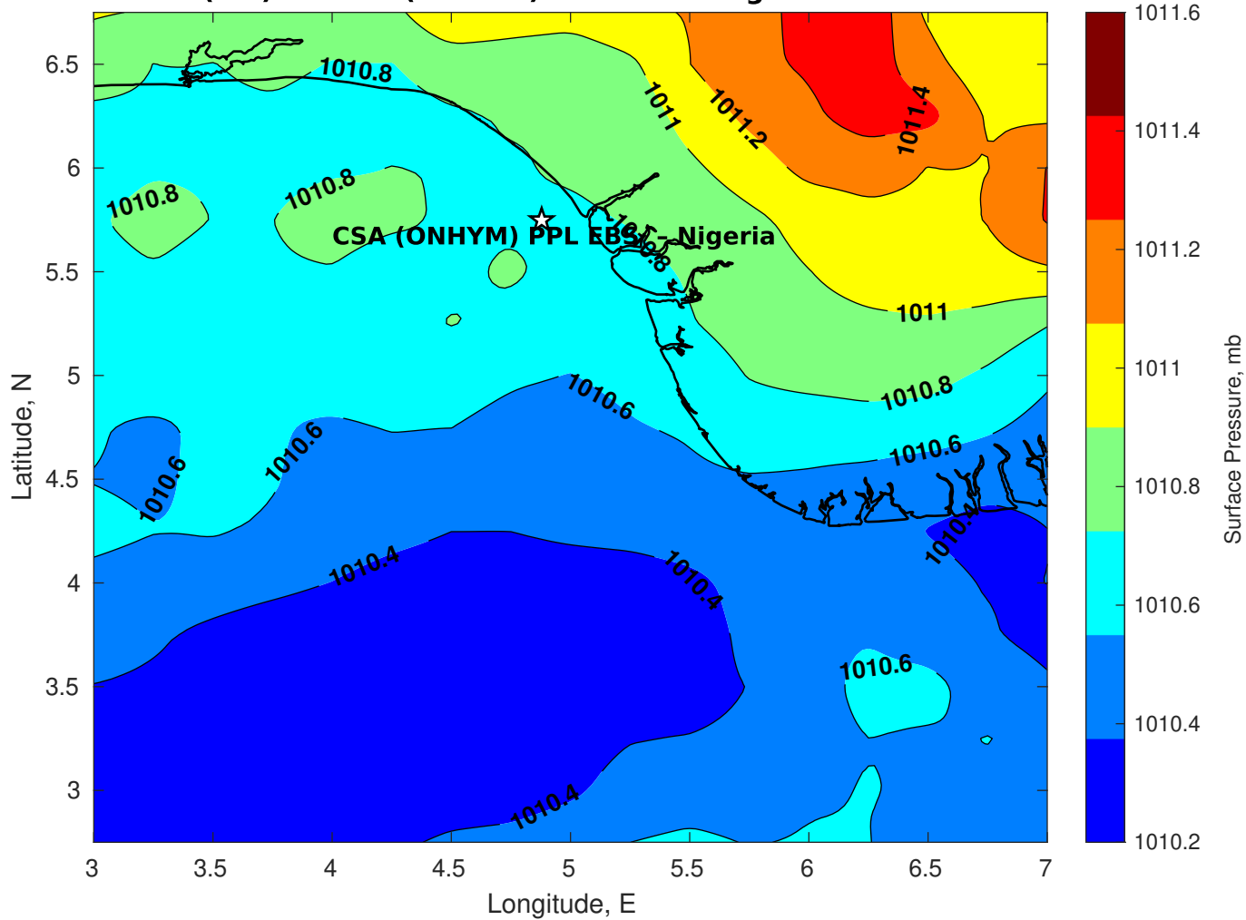
Surface Pressure (mb) for CSA (ONHYM) PPL EBS - Nigeria at 25-Dec-2025 06:00:00
