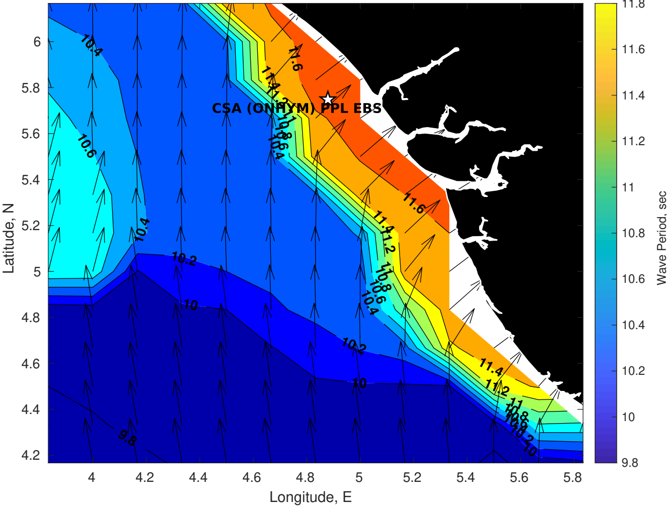
GFS Wave Period (sec) for CSA (ONHYM) PPL EBS - Nigeria at 25-Dec-2025 09:00:00
