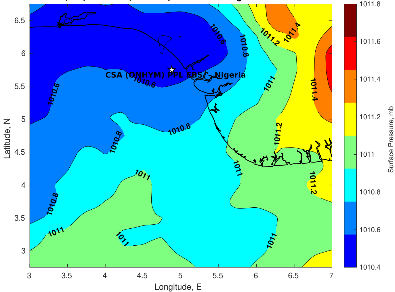
Surface Pressure (mb) for CSA (ONHYM) PPL EBS - Nigeria at 27-Dec-2025 06:00:00
