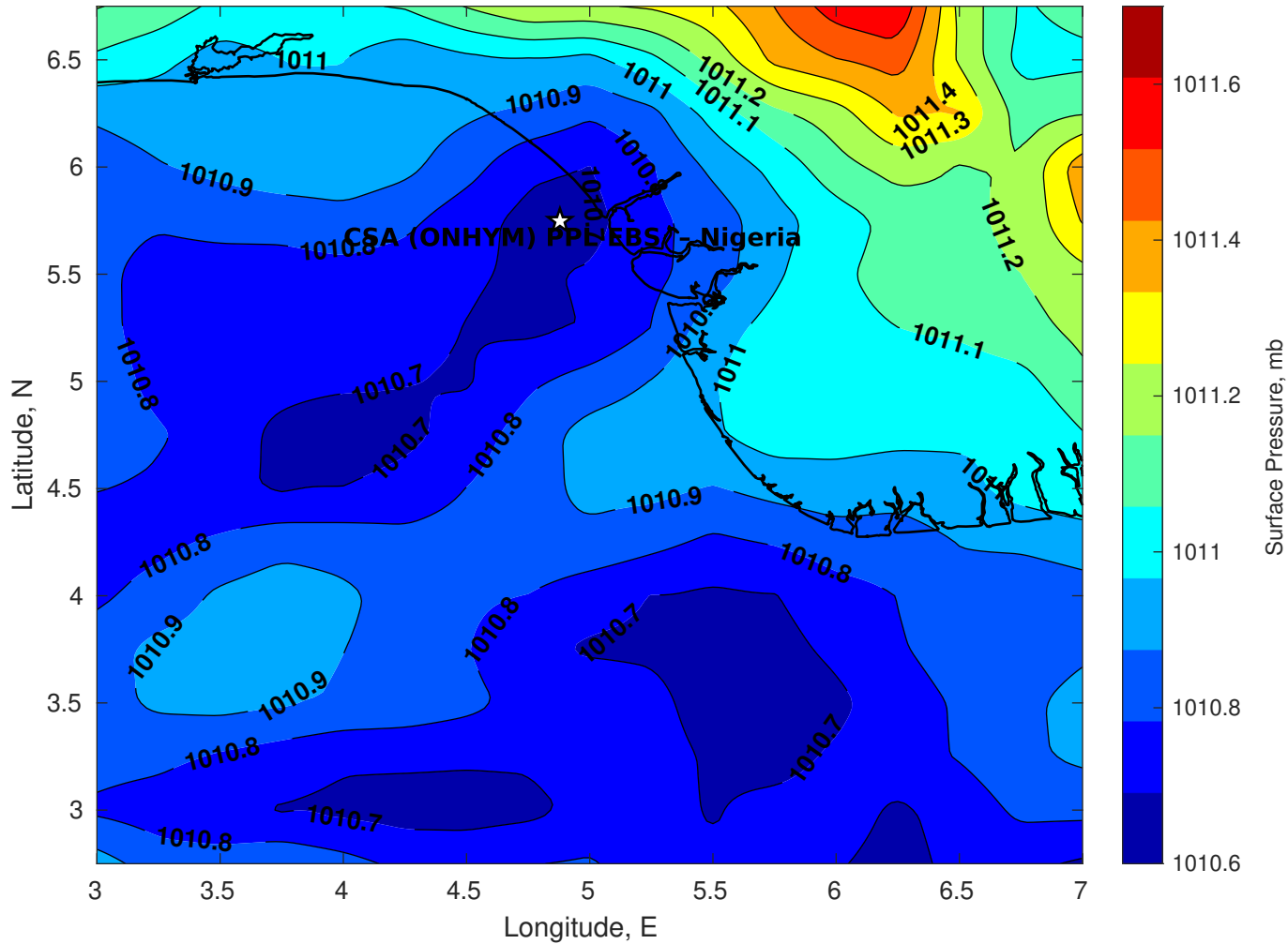
Surface Pressure (mb) for CSA (ONHYM) PPL EBS - Nigeria at 26-Dec-2025 06:00:00
