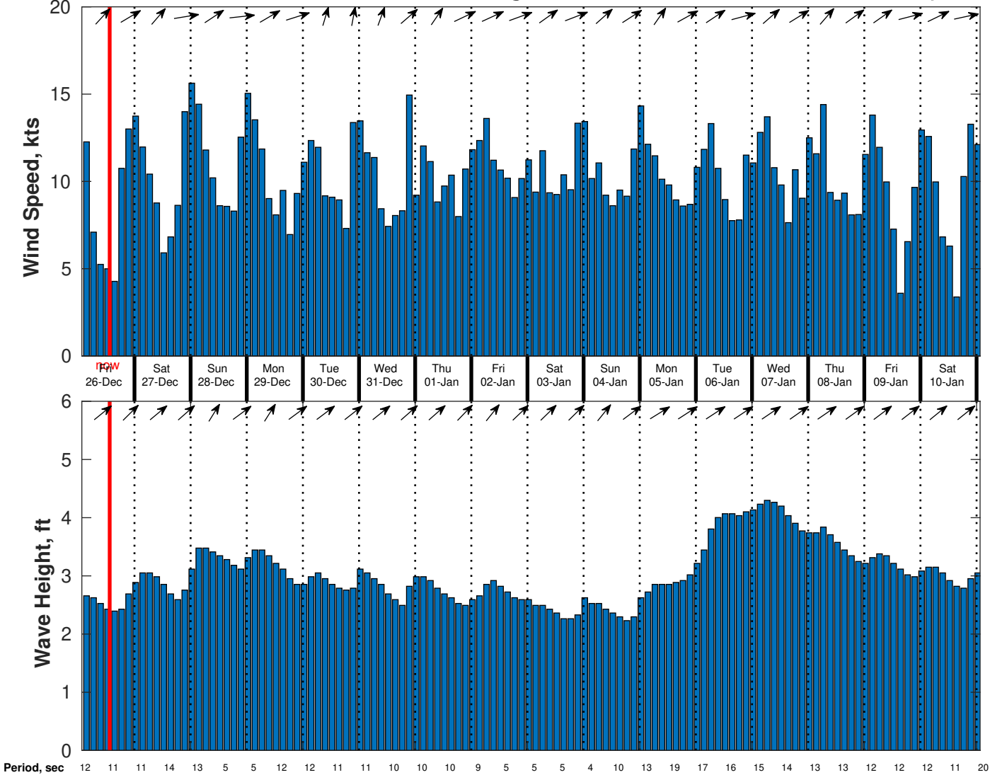
Wind & Wave Forecast for CSA (ONHYM) PPL EBS - Nigeria from 25-Dec-2025 02:00:00 to 10-Jan-2026 02:00:00
