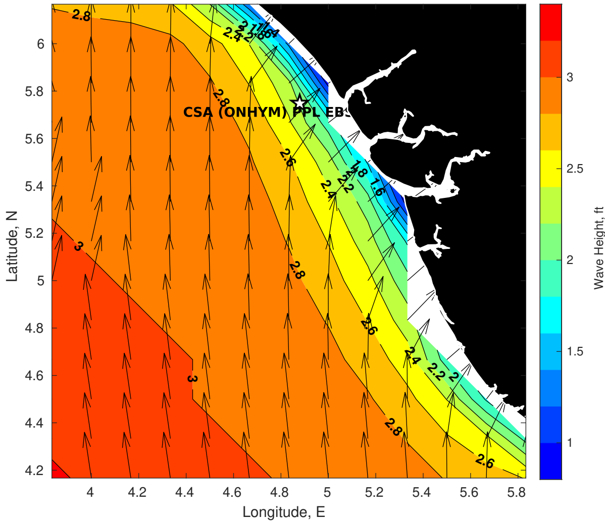
GFS Wave Height (ft) for CSA (ONHYM) PPL EBS - Nigeria at 25-Dec-2025 09:00:00
