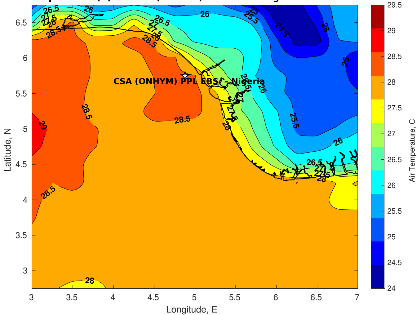
Air Temperature (C) for CSA (ONHYM) PPL EBS - Nigeria at 25-Dec-2025
