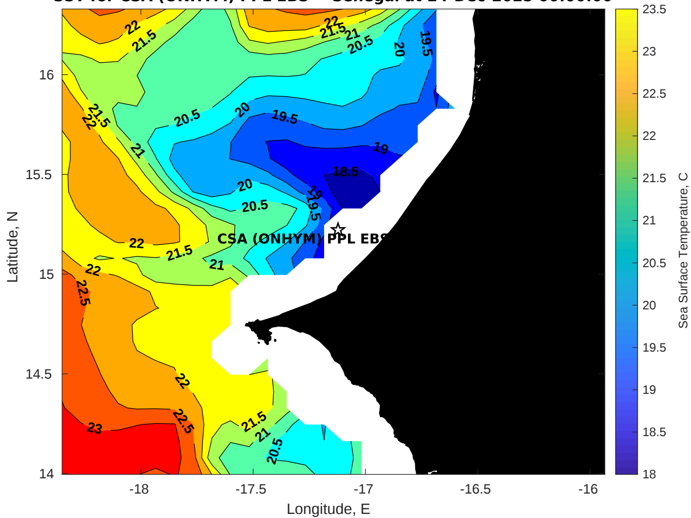
SST for CSA (ONHYM) PPL EBS - Senegal at 24-Dec-2025 00:00:00
