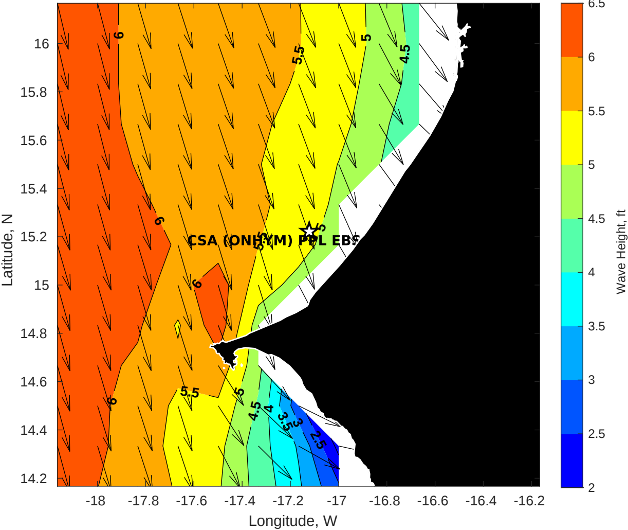
GFS Wave Height (ft) for CSA (ONHYM) PPL EBS - Senegal at 25-Dec-2025 09:00:00
