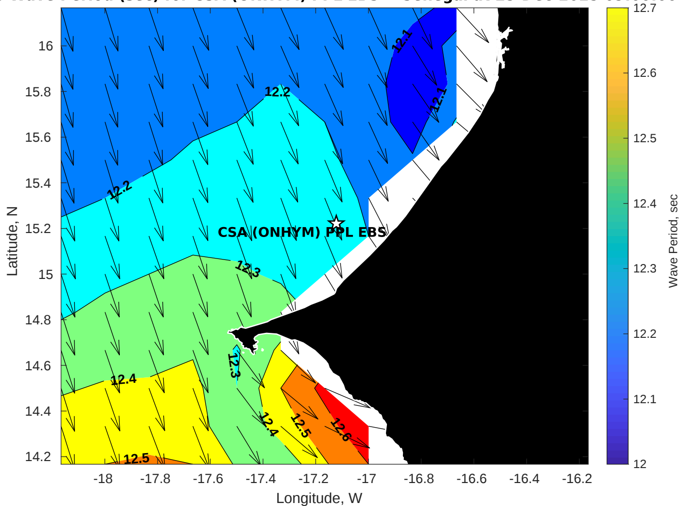
GFS Wave Period (sec) for CSA (ONHYM) PPL EBS - Senegal at 25-Dec-2025 09:00:00
