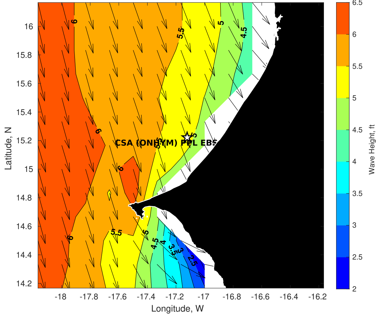
GFS Wave Height (ft) for CSA (ONHYM) PPL EBS - Senegal at 25-Dec-2025 09:00:00
