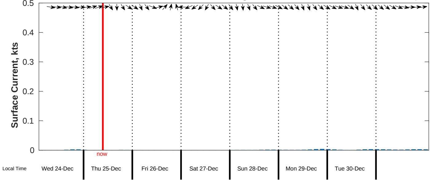
Surface Current Forecast for CSA (ONHYM) PPL EBS - Senegal from 24-Dec-2025 00:00:00 to 01-Jan-2026 00:00:00
