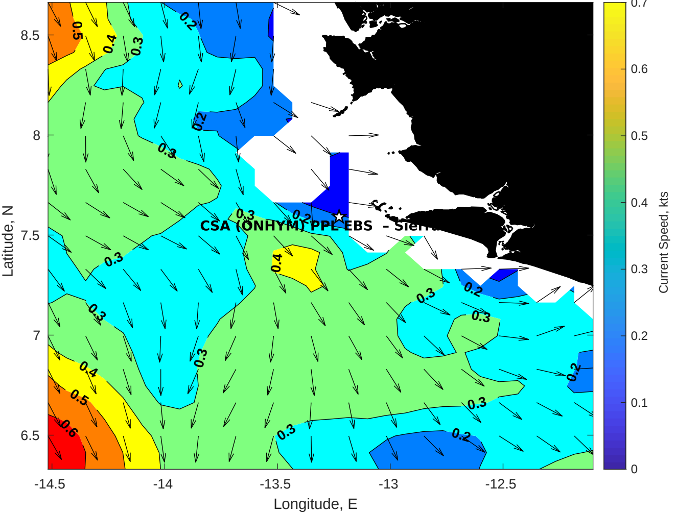
Surface Currents for CSA (ONHYM) PPL EBS - Sierra Leone at 24-Dec-2025 00:00:00
