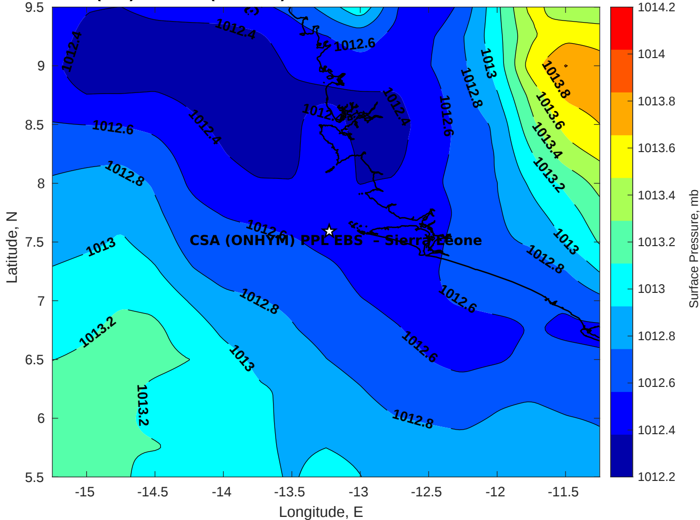
Surface Pressure (mb) for CSA (ONHYM) PPL EBS - Sierra Leone at 27-Dec-2025 00:00:00
