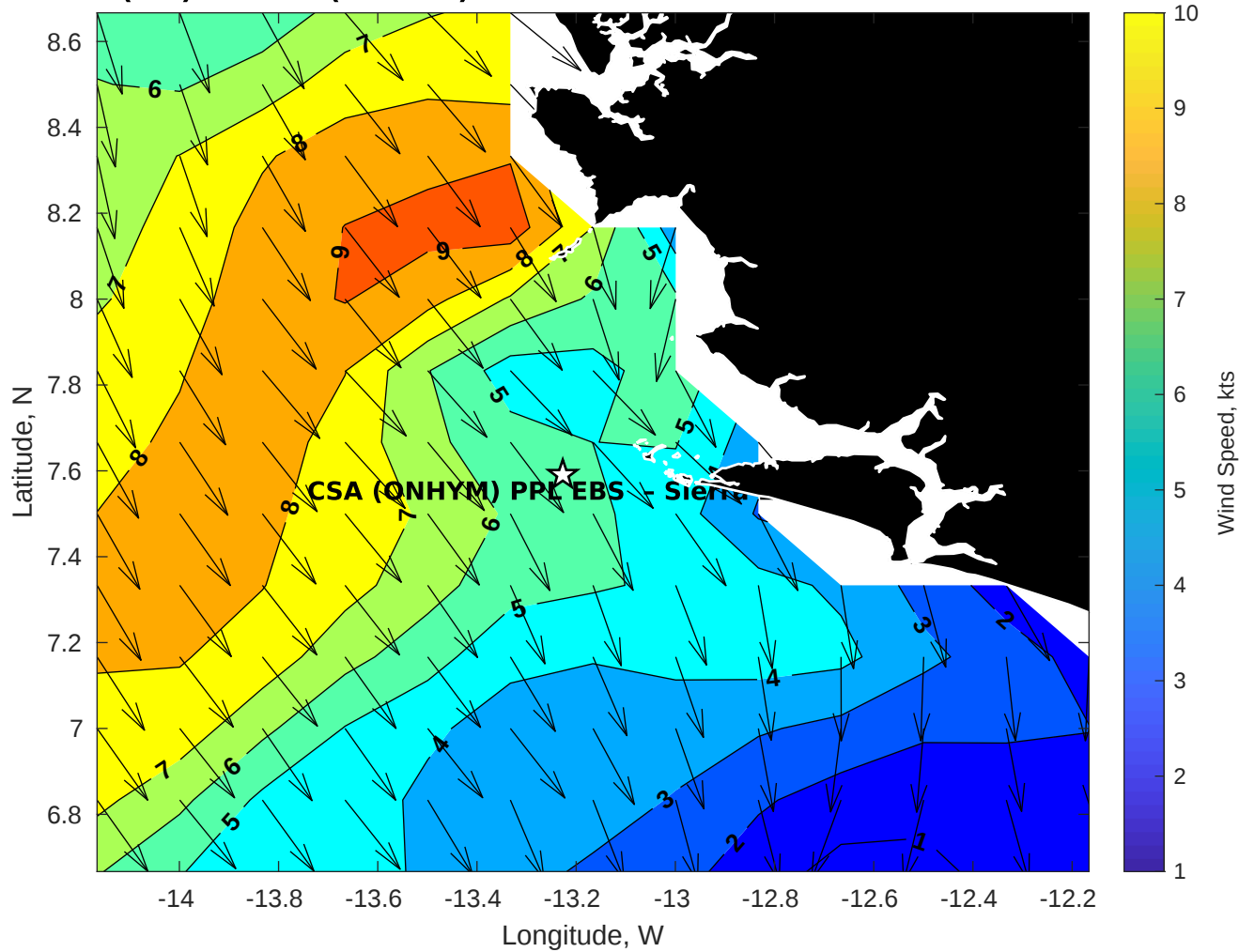
GFS Winds (kts) for CSA (ONHYM) PPL EBS - Sierra Leone at 25-Dec-2025 09:00:00
