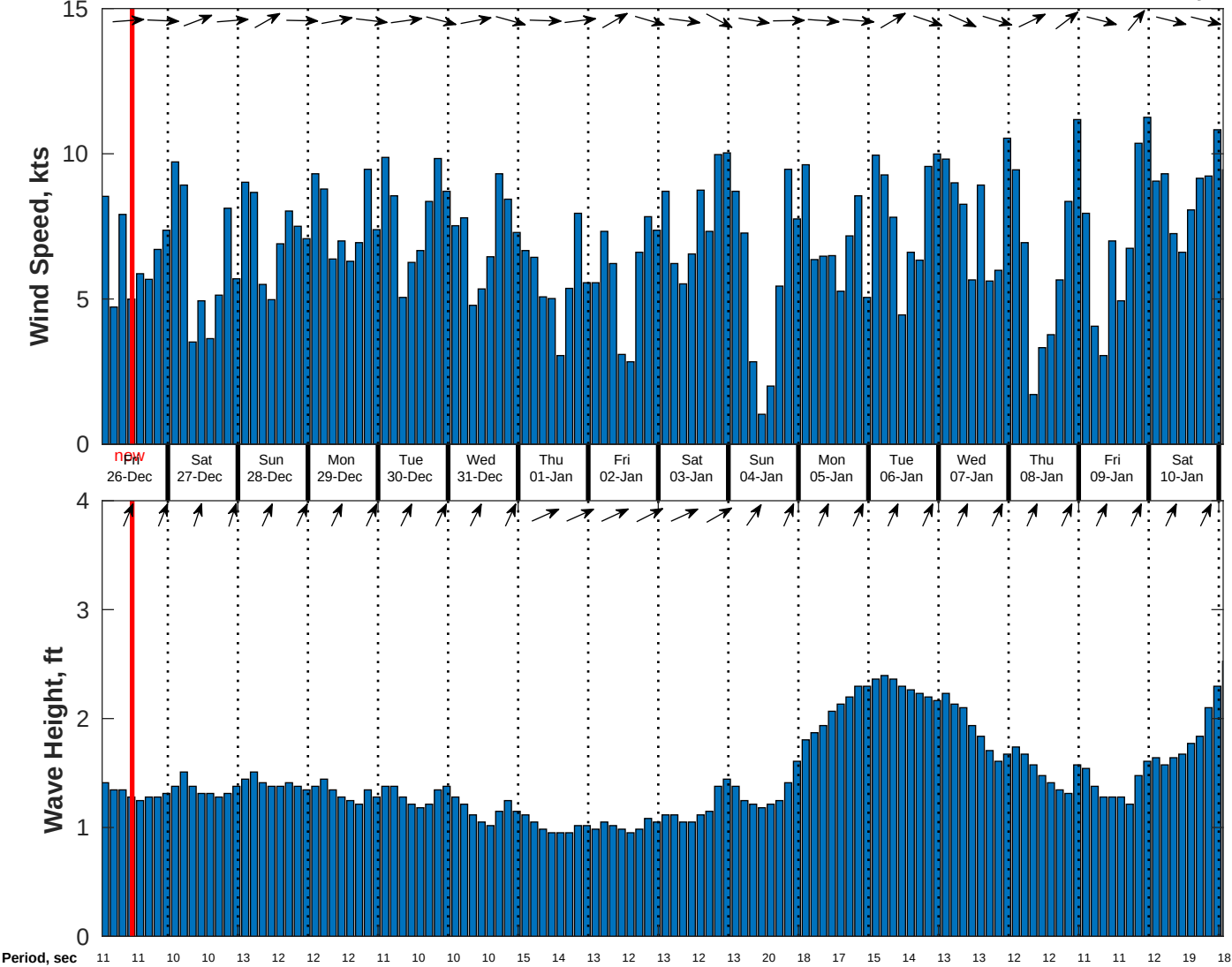
Wind & Wave Forecast for CSA (ONHYM) PPL EBS - Sierra Leone from 25-Dec-2025 01:00:00 to 10-Jan-2026 01:00:00
