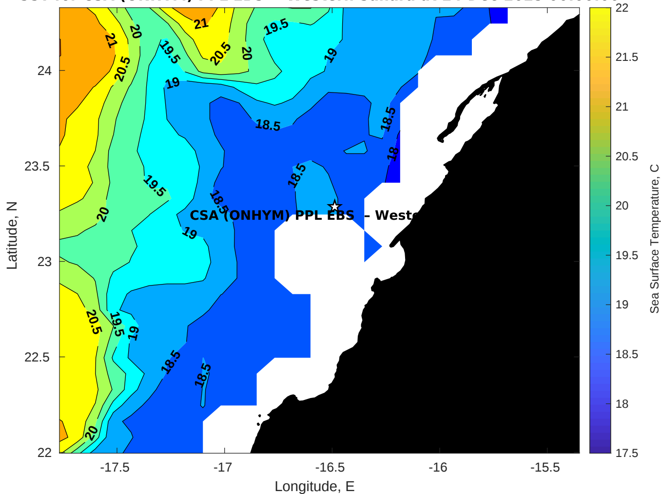
SST for CSA (ONHYM) PPL EBS - Western Sahara at 24-Dec-2025 00:00:00
