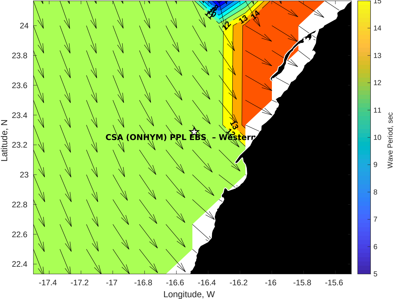
GFS Wave Period (sec) for CSA (ONHYM) PPL EBS - Western Sahara at 25-Dec-2025 09:00:00
