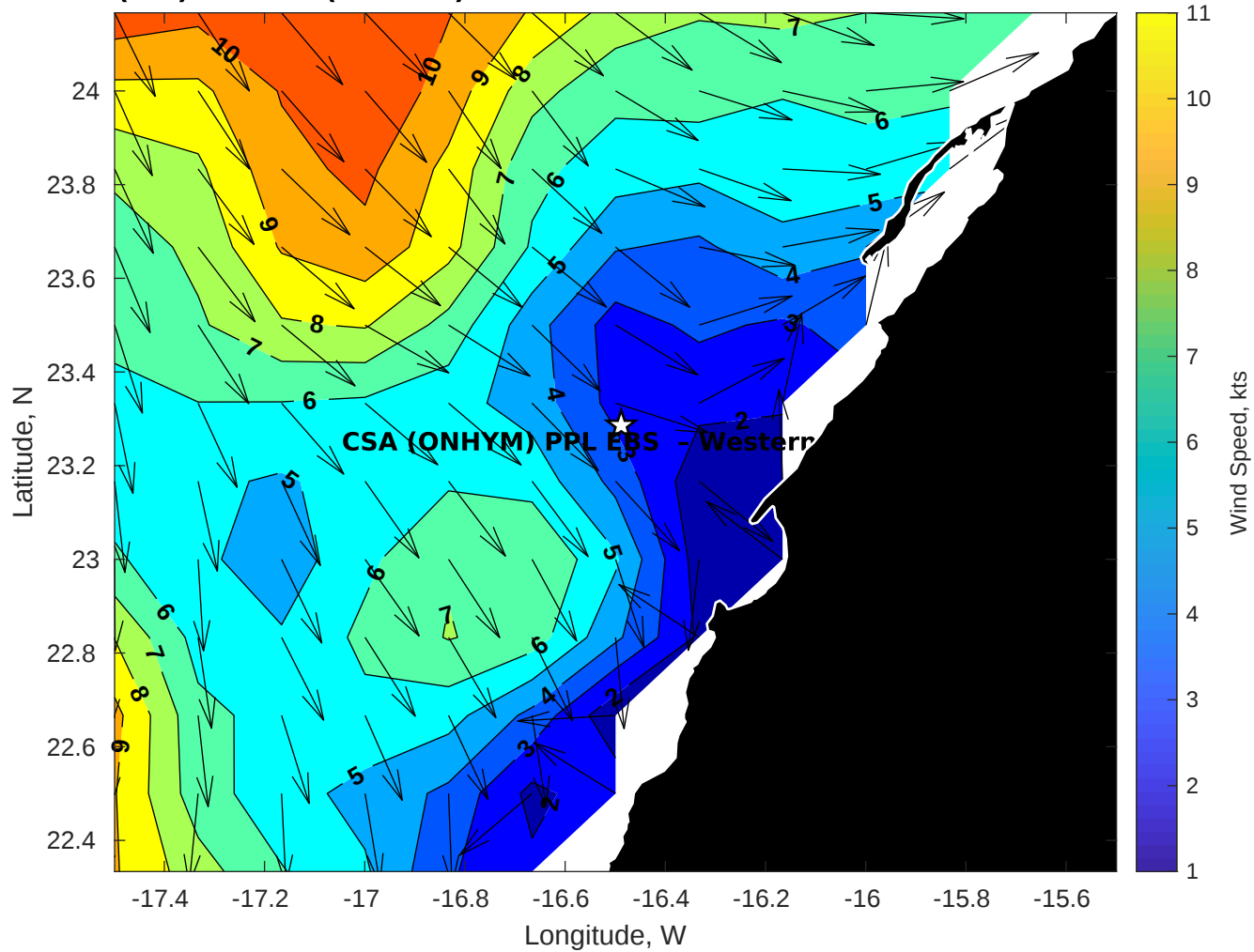
GFS Winds (kts) for CSA (ONHYM) PPL EBS - Western Sahara at 25-Dec-2025 09:00:00
