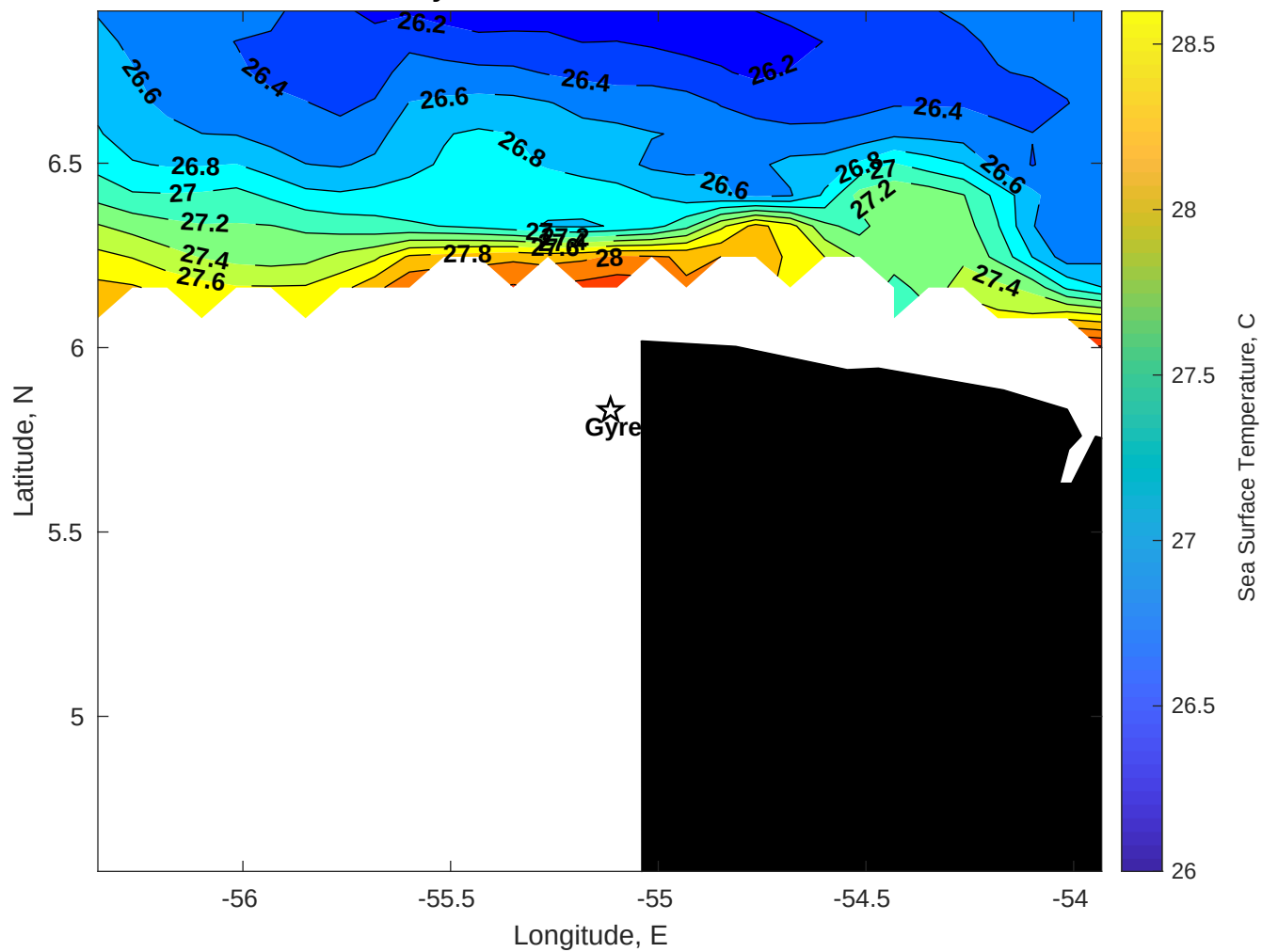
SST for Gyre at 24-Dec-2025 00:00:00
